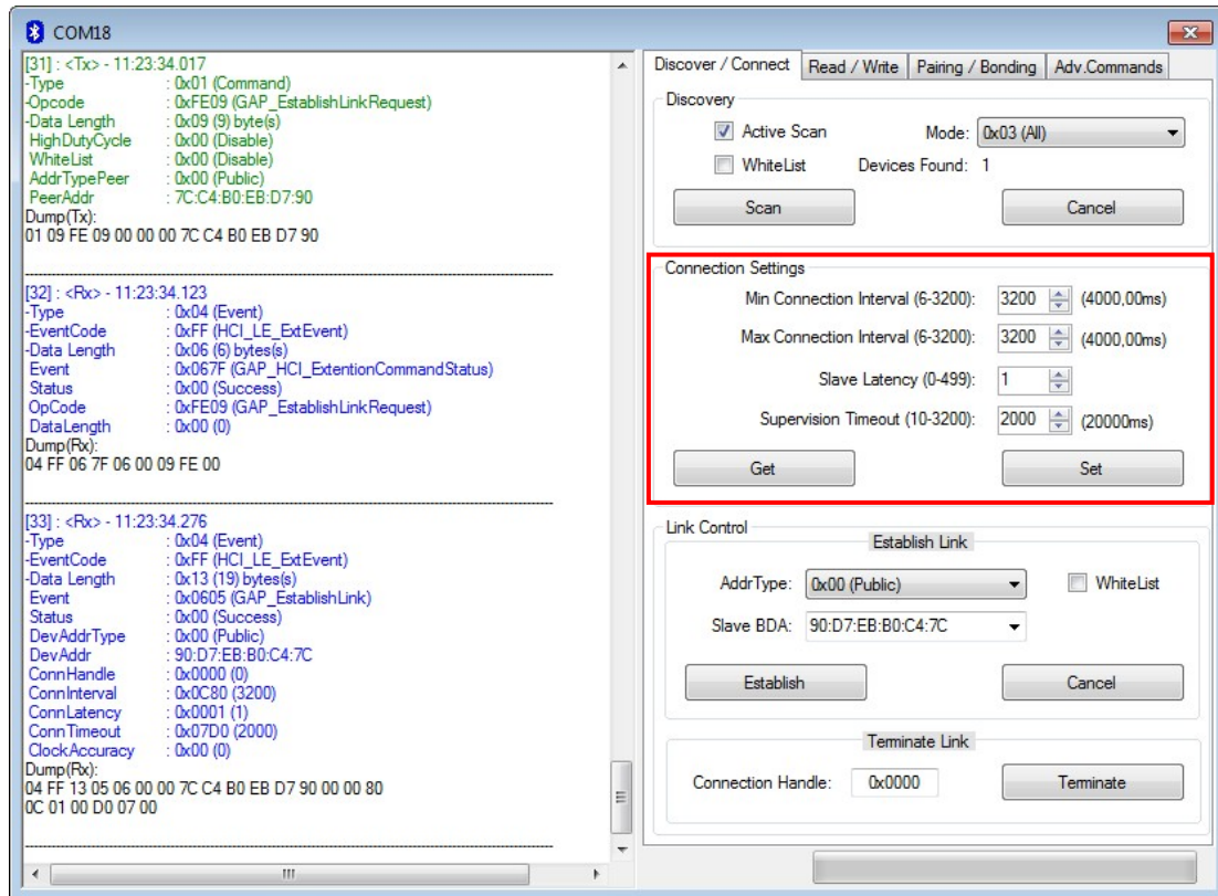
Figure 16- BTool set up for 8 Second Effective Connection Interval
