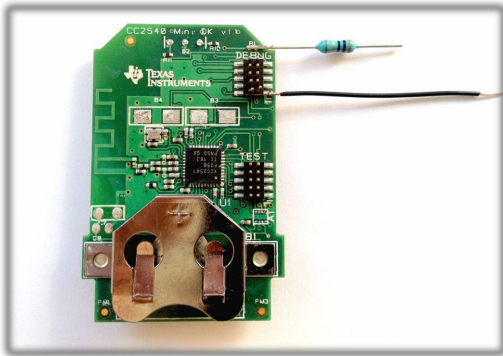
Figure 15- Keyfob Board with Peripherals Removed
