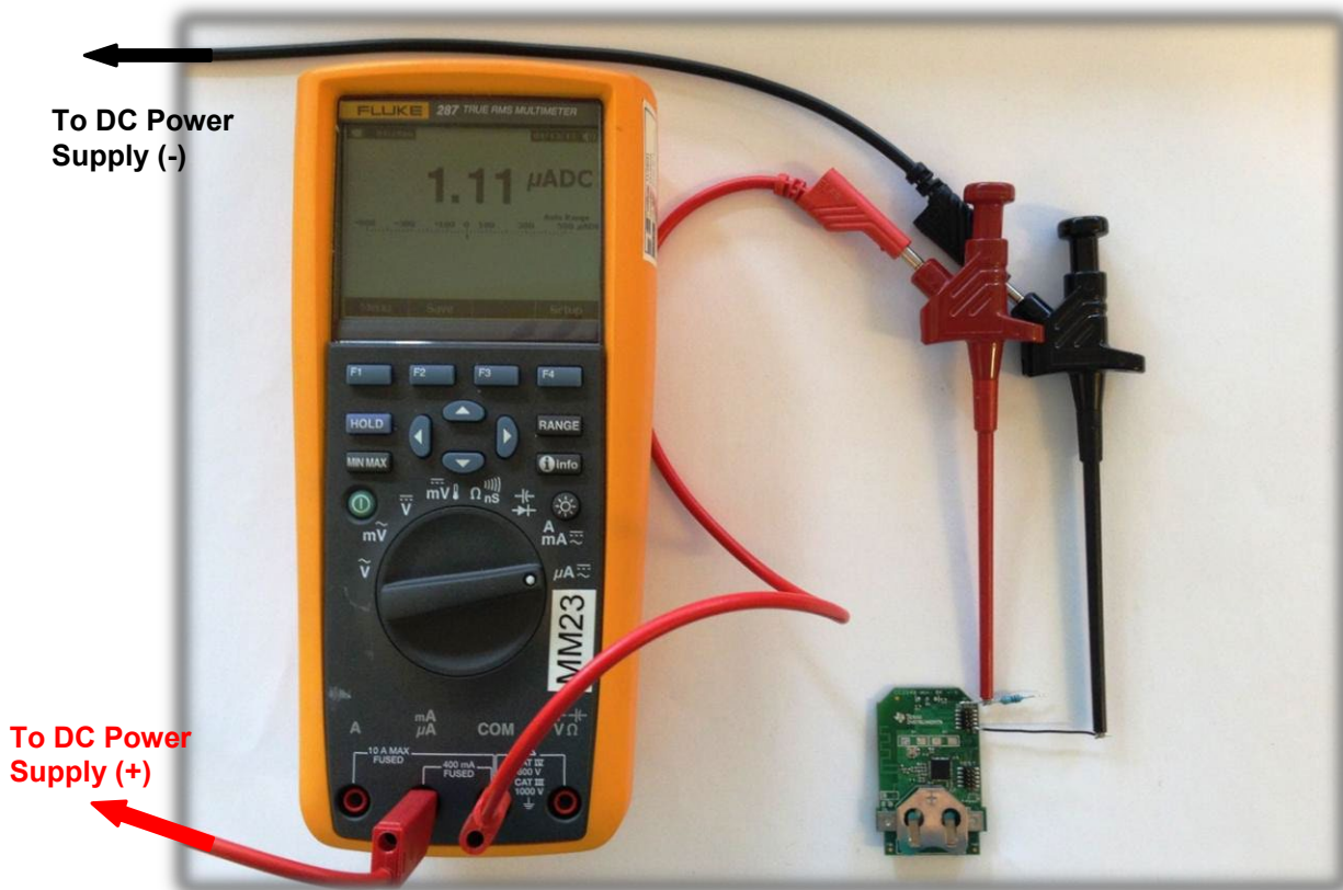
Figure 17- 1 \mu A PM2 Sleep Current Measured on Keyfob
