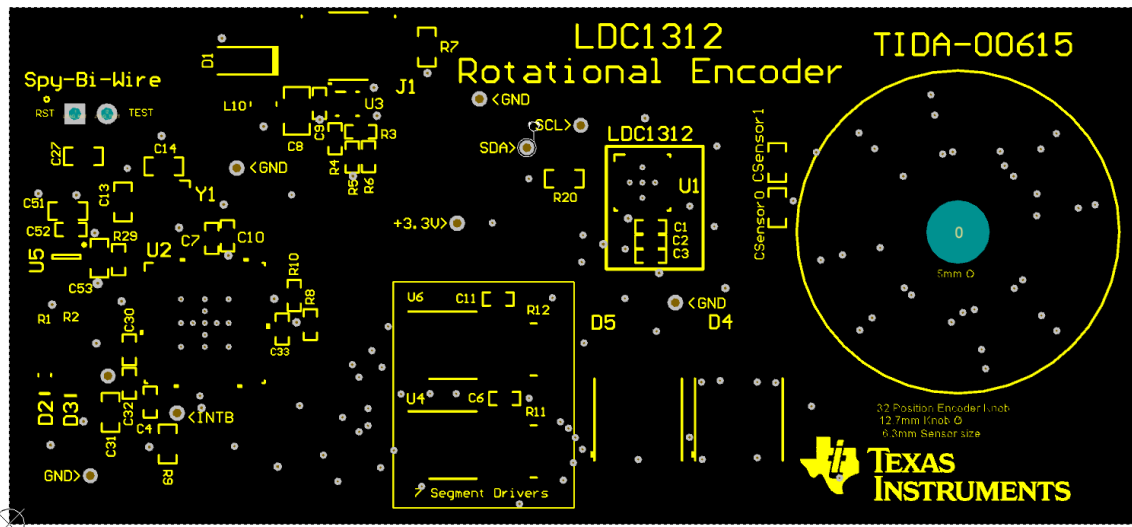
Figure 2: Sensor PCB Top Silkscreen
