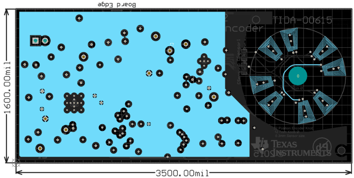
Figure 5: Sensor PCB Midlayer2 Routing
