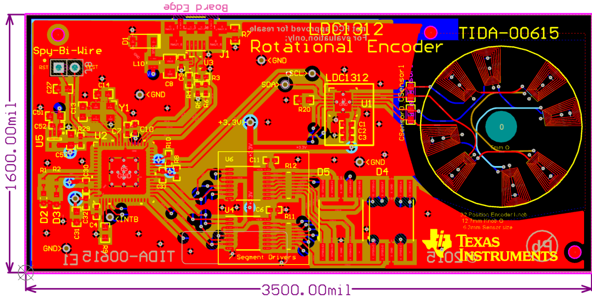
Figure 1: Multi-layer Sensor Print
