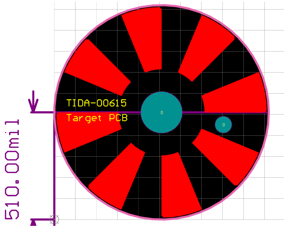
Figure 7: Target PCB Top Layer Routing
