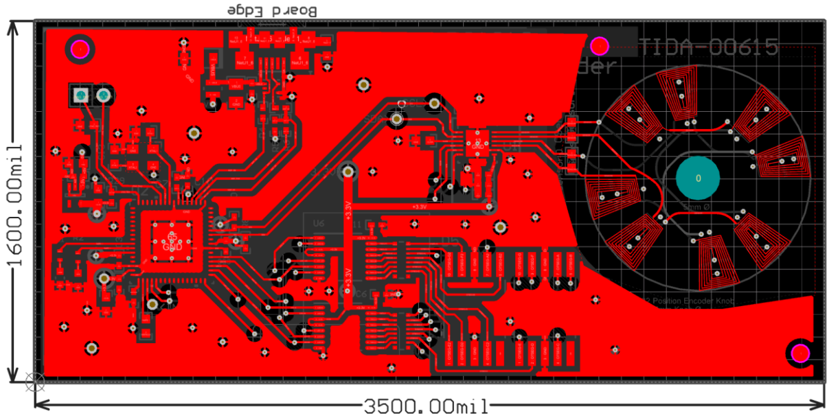
Figure 3: Sensor PCB Top Layer Routing
