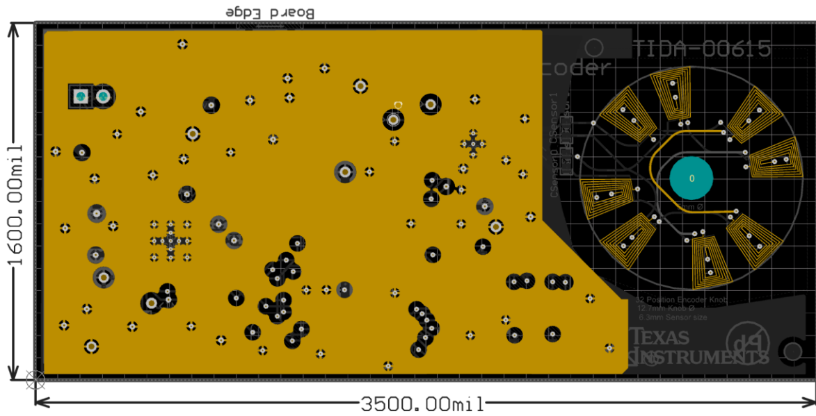
Figure 4: Sensor PCB Midlayer1 Routing
