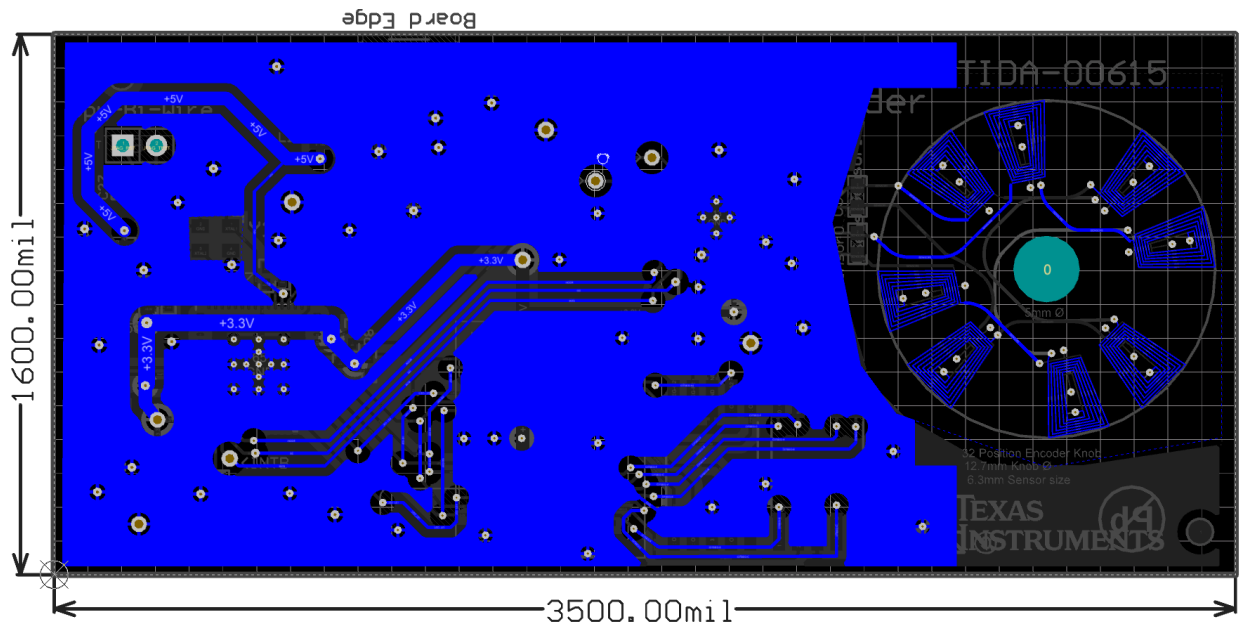
Figure 6: Sensor PCB Bottom Layer Routing
