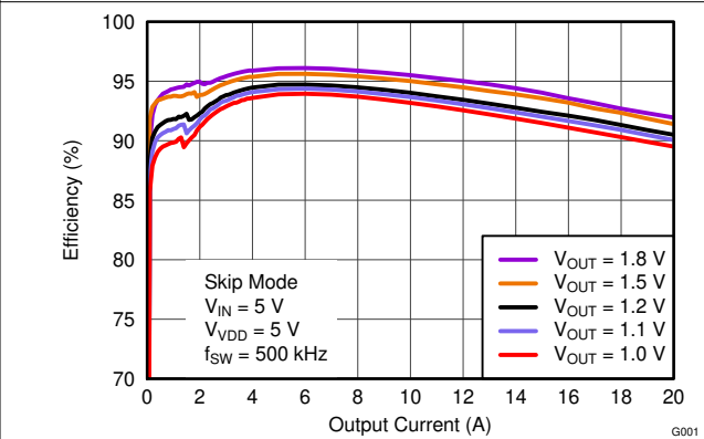
图 6-33. Efficiency vs Output Current
