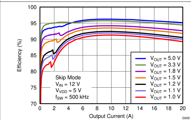
图 6-31. Efficiency vs Output Current
