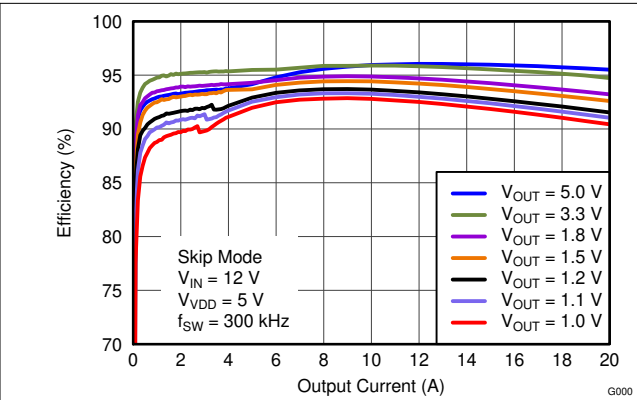
图 6-29. Efficiency vs Output Current
