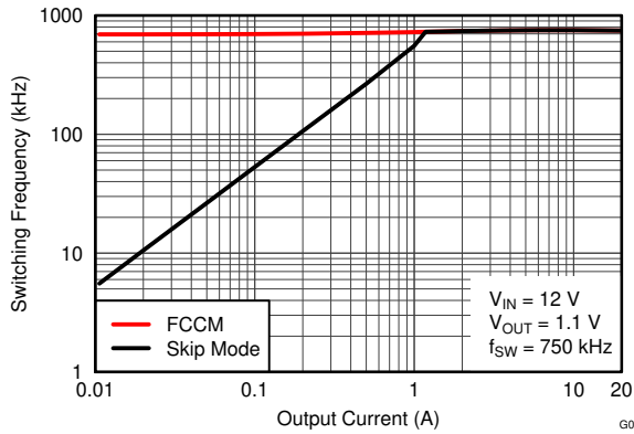
图 6-7. Switching Frequency vs. Output Current
