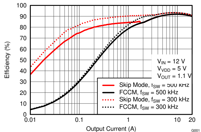
图 6-12. Efficiency vs Output Current
