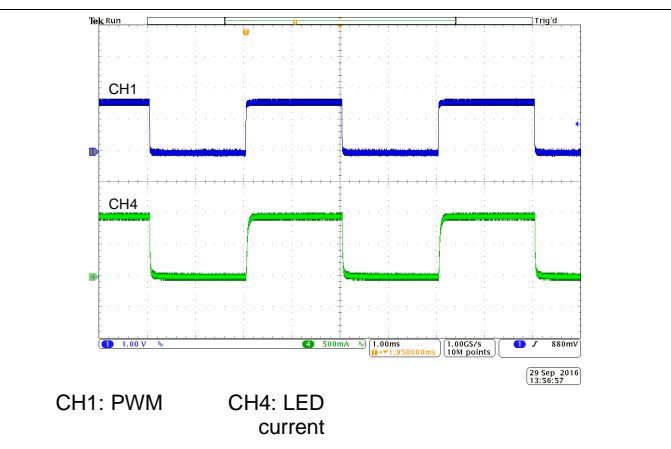
图 46. PWM Dimming With 50% Duty Cycle and 250 Hz
