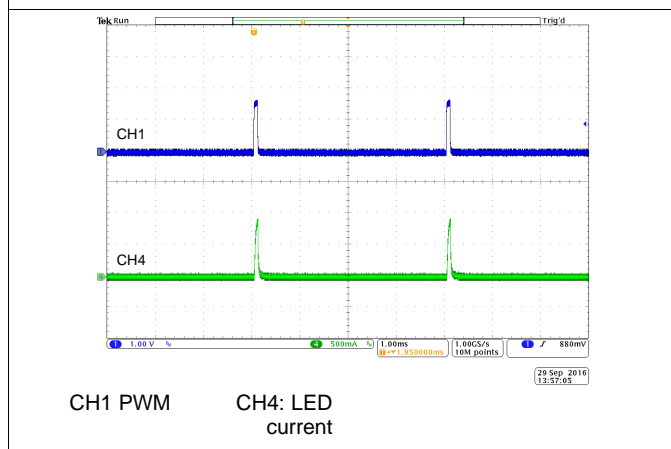
图 45. PWM Dimming With 2% Duty Cycle and 250 Hz
