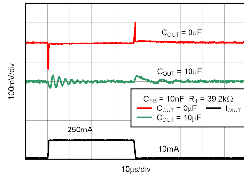
图 5-52. TPS73201 Load Transient, Adjustable Version
