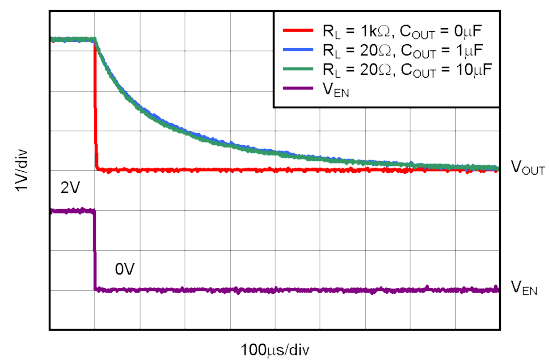
图 5-42. TPS73233 Turn-Off Response
