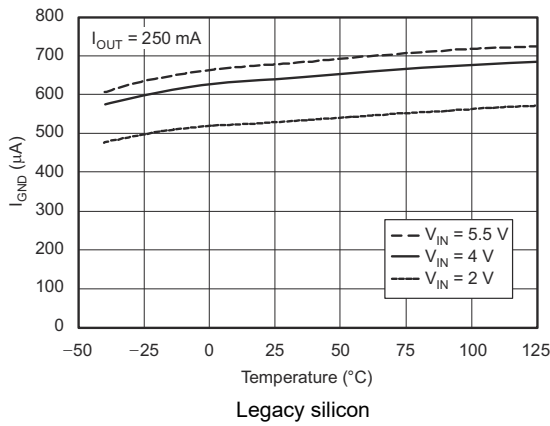
图 5-13. Ground Pin Current vs Temperature
