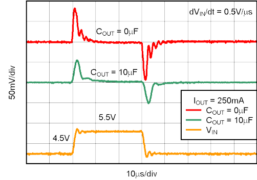
图 5-38. TPS73233 Line Transient Response
