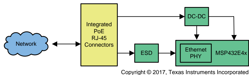
图 1. PoE for Connected IoT Block Diagram
