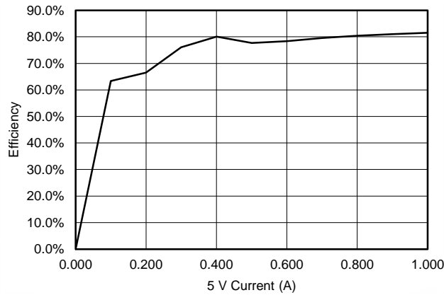
图 5. Efficiency Chart
