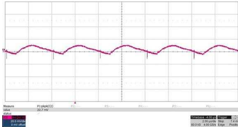
图 6. Ripple Voltage on 5-V Load
