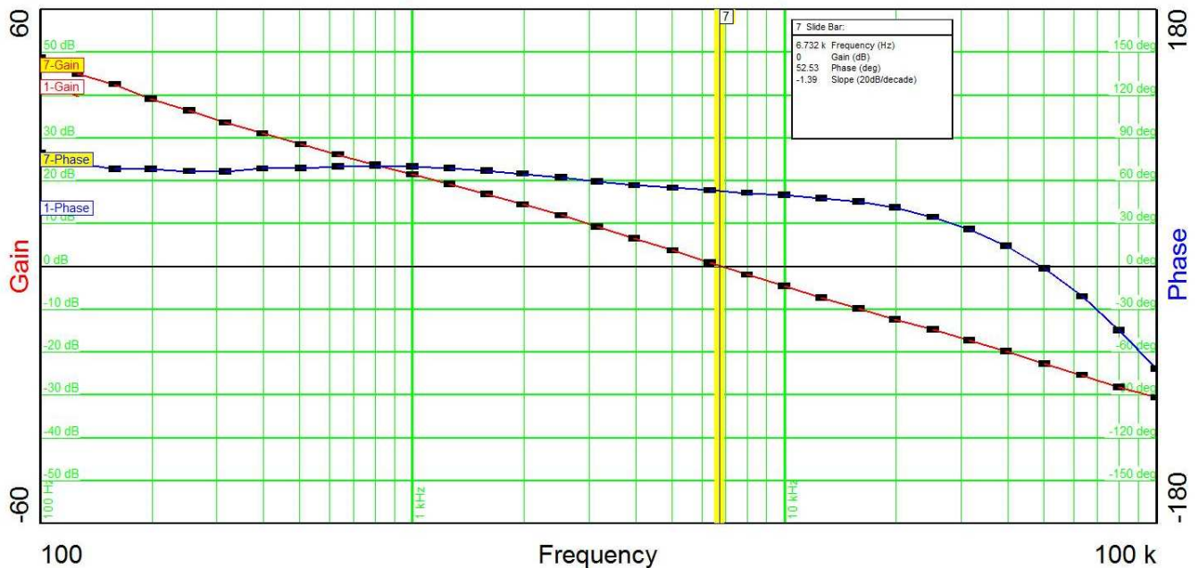
图 11. Control Loop Gain Stability
