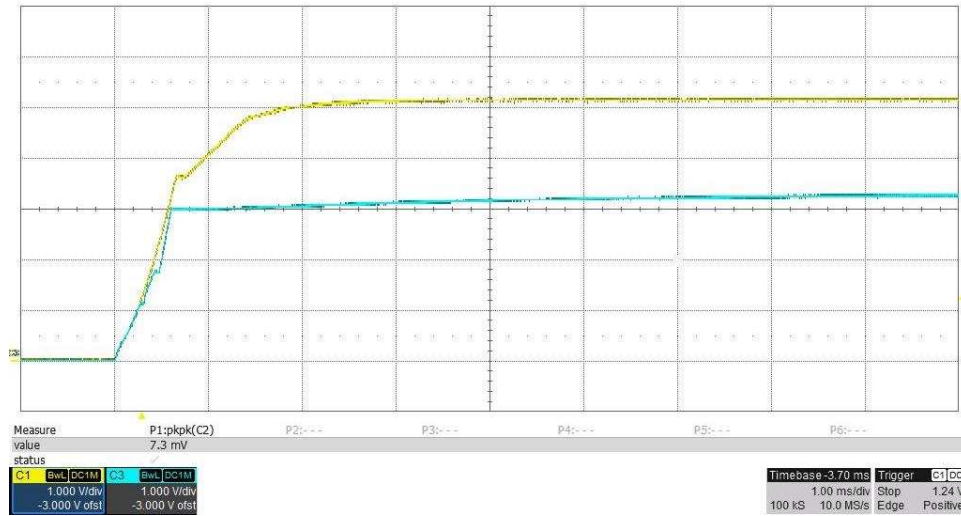
图 4. Start-Up Under Load Conditions
