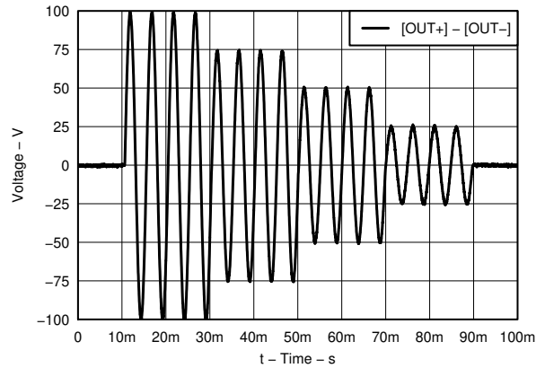
6-16. Example Waveform – Amplitude
