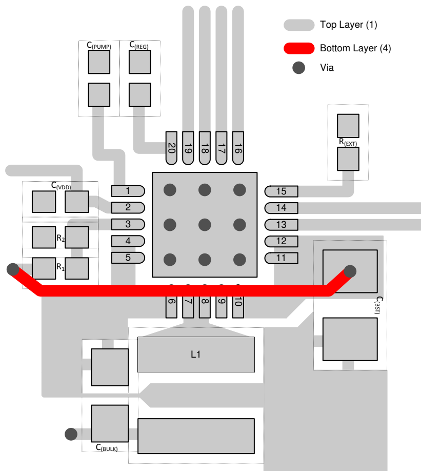
10-1. Layout Example with a 4-Layer Board
