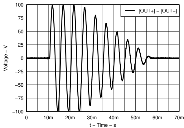
6-17. Example Waveform – Envelope Down
