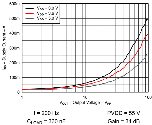
6-5. Supply Current vs Output Voltage
