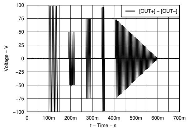
6-20. Example Waveform – Pinball Effect
