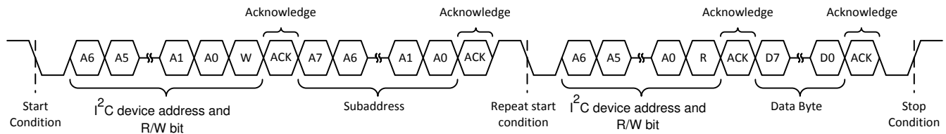
7-13. Single-Byte Read Transfer
