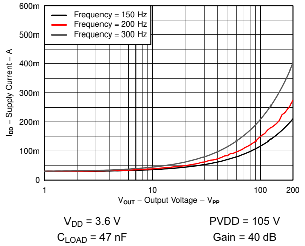
6-4. Supply Current vs Output Voltage
