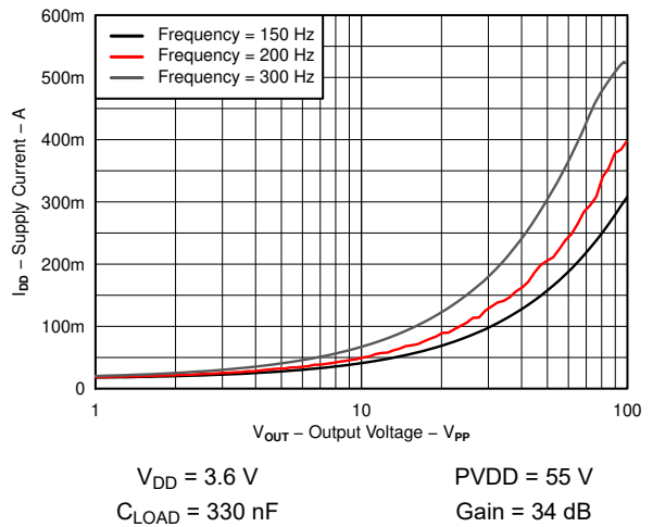
6-6. Supply Current vs Output Voltage
