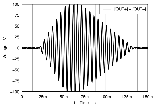
6-19. Example Waveform – Envelope Up and Down
