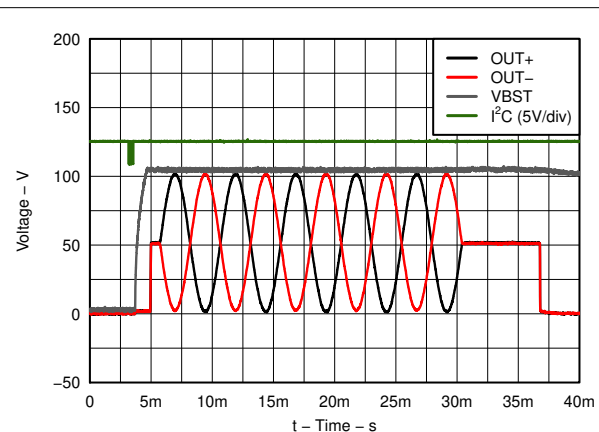
8-4. Typical Waveform
