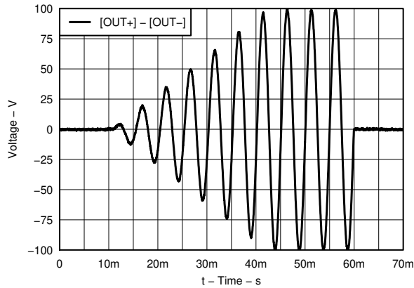
6-15. Example Waveform – Envelope Up
