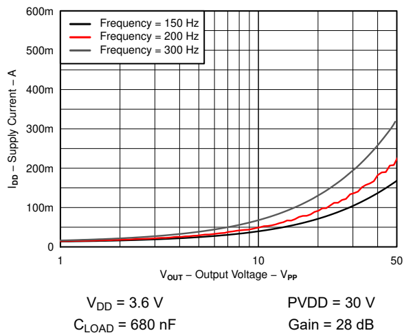
6-8. Supply Current vs Output Voltage
