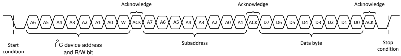
7-11. Single-Byte Write Transfer
