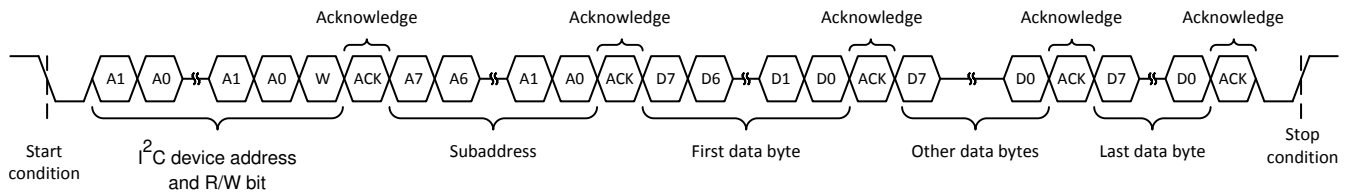
7-12. Multiple-Byte Write Transfer
