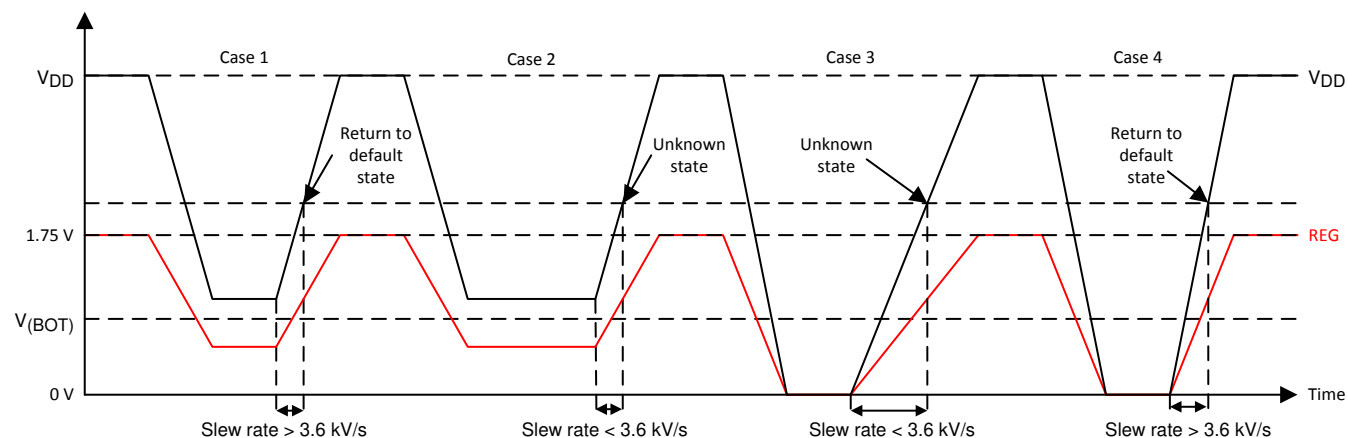
Figure 7-2. Brownout Behavior
