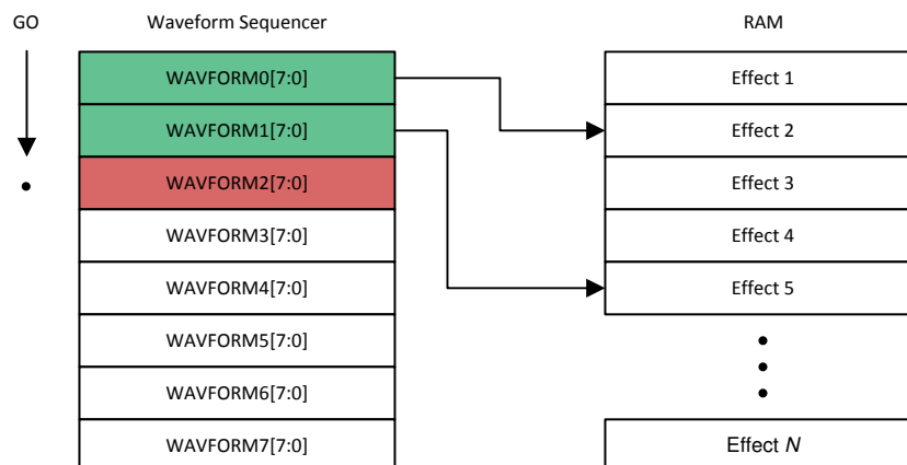
7-9. Waveform Sequencer
