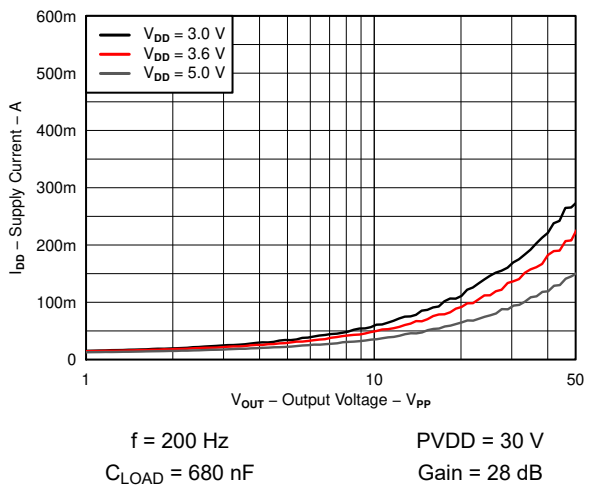
6-7. Supply Current vs Output Voltage
