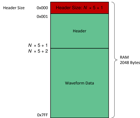
7-5. RAM Structure
