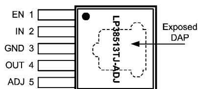
Top View TO-263 THIN 5 Pin Package
