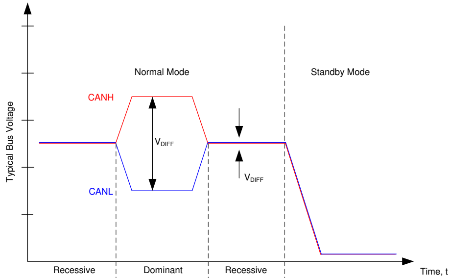
7-4. Bus States
