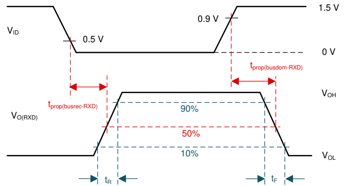
図 6-3. Receiver Test Circuit and Measurement
