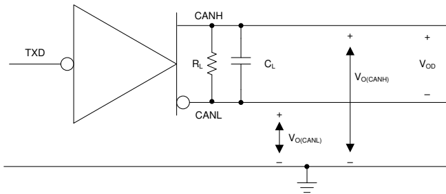
図 6-2. Driver Test Circuit and Measurement
