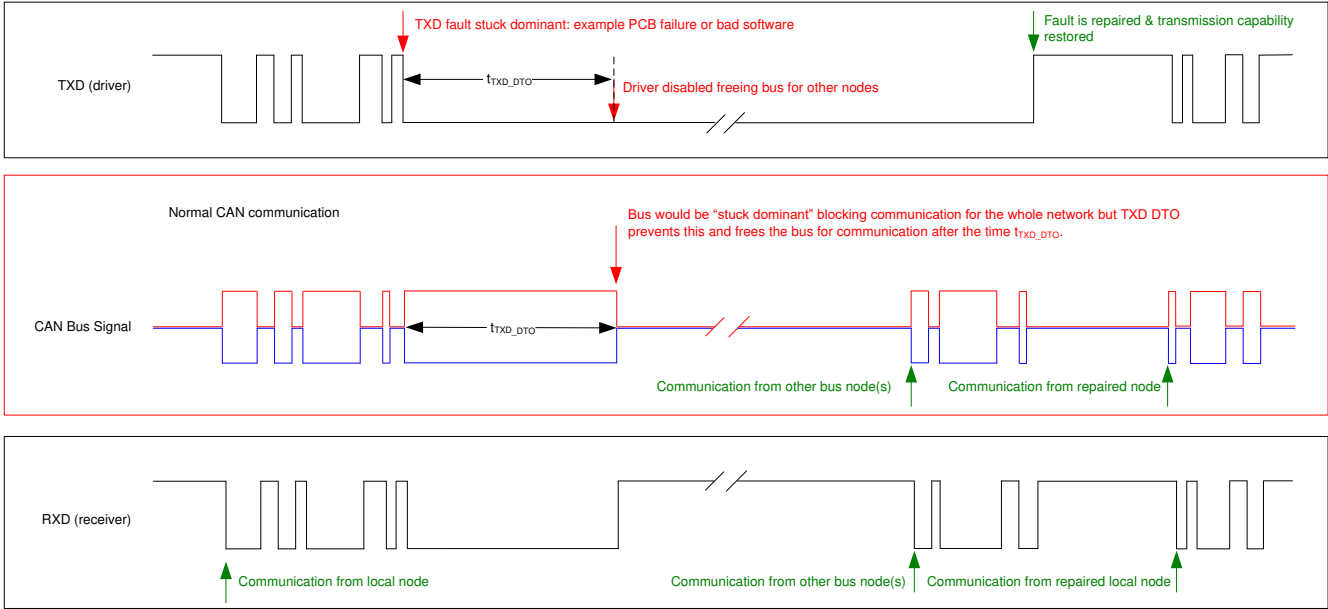
7-6. Example Timing Diagram for TXD Dominant Timeout
