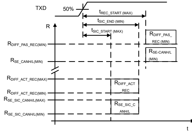
図 7-2. TX based SIC
