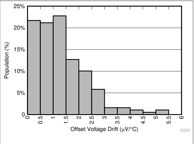
6-2. Offset Voltage Drift Distribution
