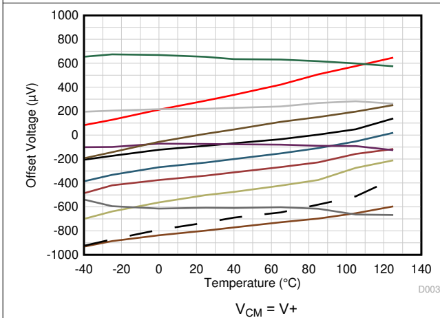
6-3. Offset Voltage vs Temperature
