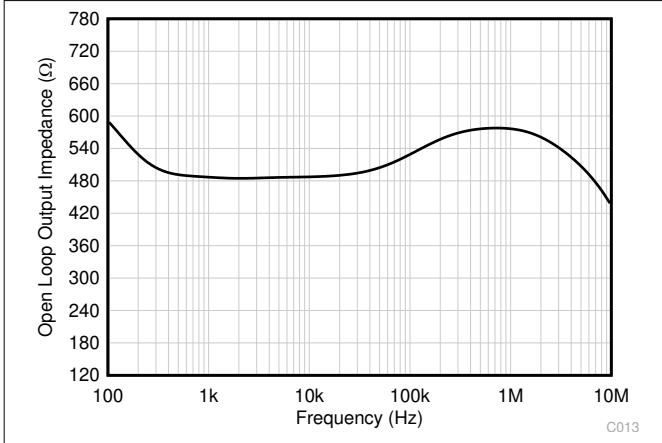
6-25. Open-Loop Output Impedance vs Frequency
