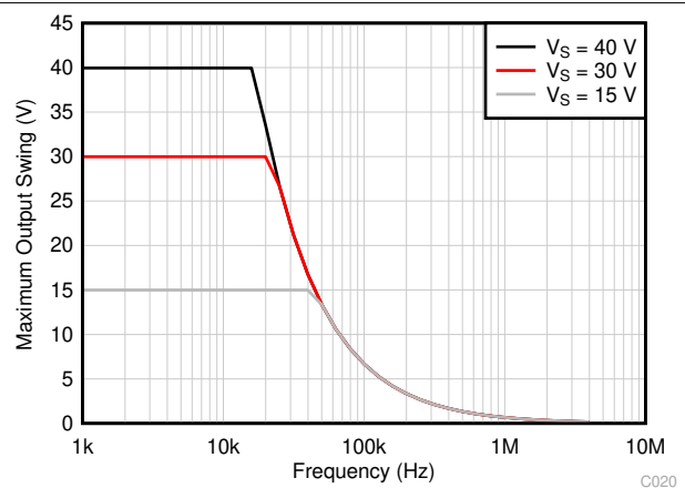
6-38. Maximum Output Voltage vs Frequency
