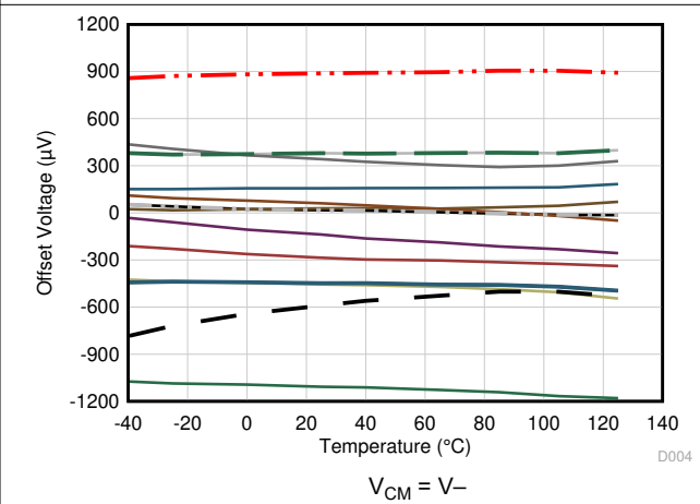
6-4. Offset Voltage vs Temperature
