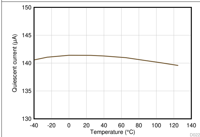
6-23. Quiescent Current vs Temperature
