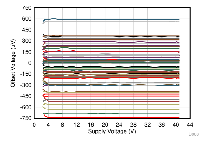
6-6. Offset Voltage vs Power Supply
