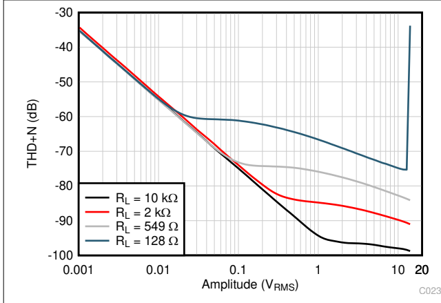
6-21. THD+N vs Output Amplitude
