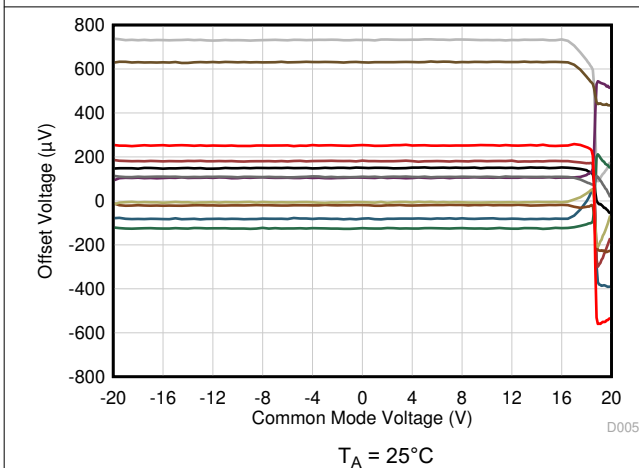
6-5. Offset Voltage vs Common-Mode Voltage
