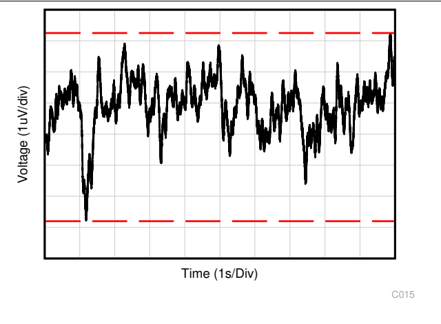
6-18. 0.1-Hz to 10-Hz Noise
