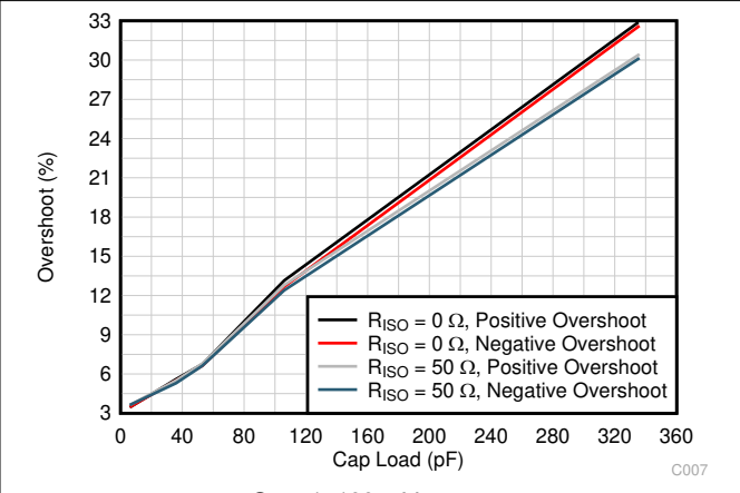
6-26. Small-Signal Overshoot vs Capacitive Load
