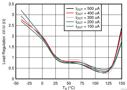
TMP23x-Q1: V_{DD} = 2.3 V, C_{LOAD} = 1000 pF
