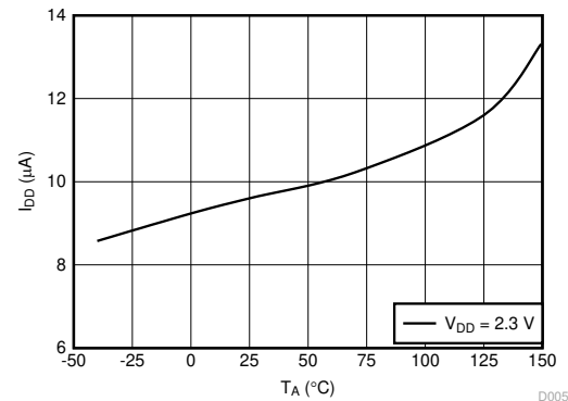
TMP23x-Q1: I_{OUT} = 0 \mu\text{A} , C_{LOAD} = 1000 pF
