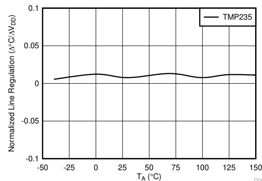
TMP23x-Q1: V_{DD} = 2.3 to 5.5 V, I_{OUT} = 0 \mu\text{A} , C_{LOAD} = 1000 pF
