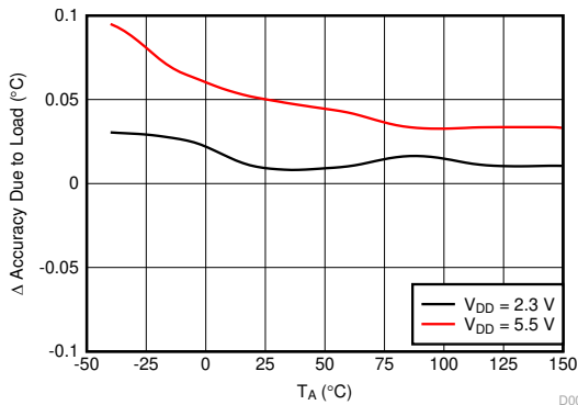
TMP23x-Q1: I_{OUT} = from 0 \mu\text{A} to 100 \mu\text{A} , C_{LOAD} = 1000 pF
