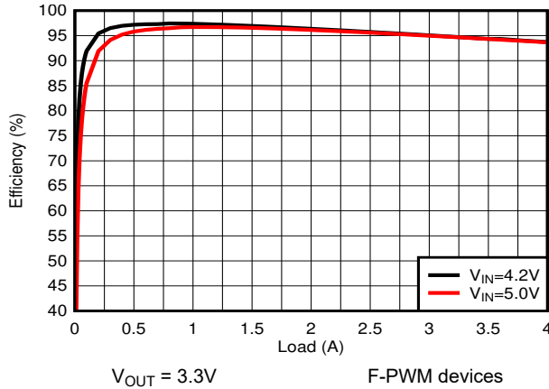
8-21. PWM Efficiency
