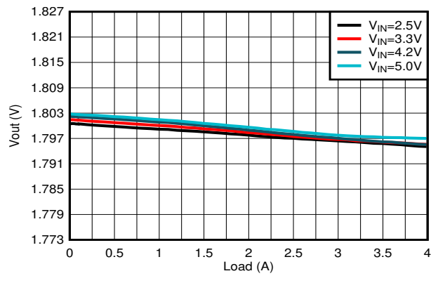
8-14. Load Regulation
