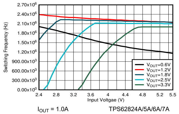
8-26. Switching Frequency
