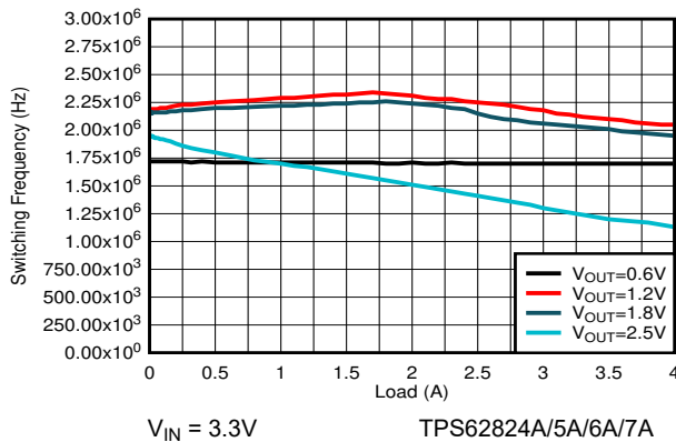
8-25. Switching Frequency
