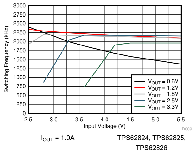
8-24. Switching Frequency
