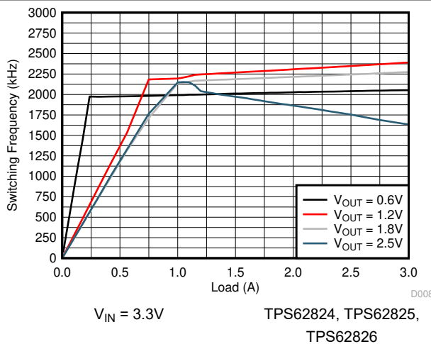
8-23. Switching Frequency
