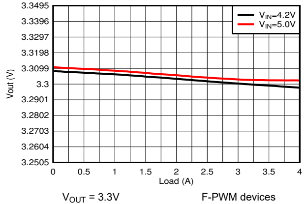
8-22. Load Regulation
