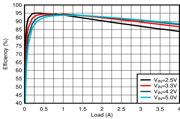
8-11. Efficiency
