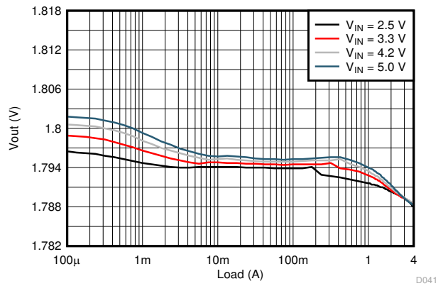
8-10. Load Regulation
