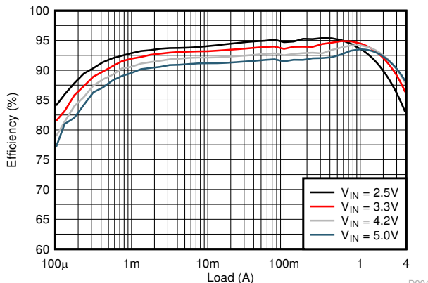
8-9. PWM Efficiency
