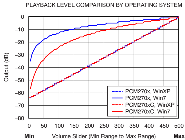
Figure 1. Playback Level Comparison of PCM270x/270xC Devices by Operating System
