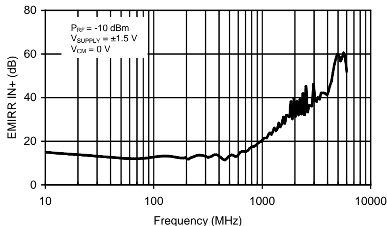
Figure 1. TLV2761 EMIRR IN+ vs Frequency
