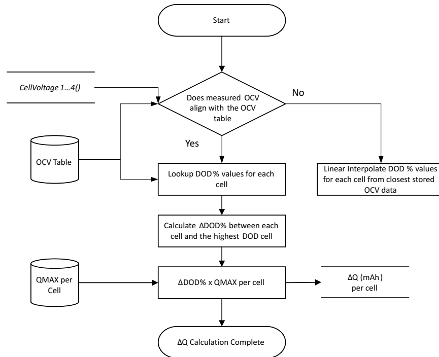
Figure 7-3. ΔQ Calculation
