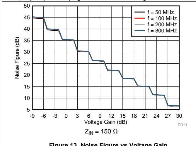
Figure 13. Noise Figure vs Voltage Gain
