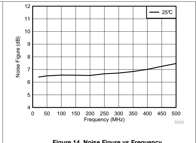
Figure 14. Noise Figure vs Frequency
