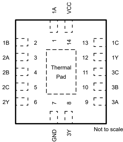
Figure 4-1. SN74LVC11A-Q1 BQA Package, 14-Pin WQFN (Top View)
