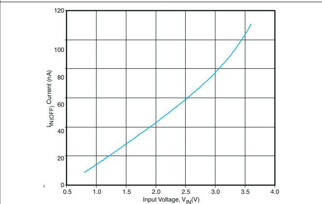
Figure 7-6. I_{IN(OFF)} vs V_{IN} ( V_{ON} = 0 V)
