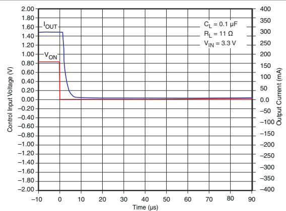
Figure 7-34. t_{OFF} Response
