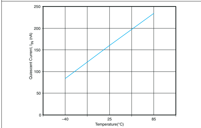
Figure 7-5. Quiescent Current vs Temperature ( V_{IN} = 3.3 V, I_{OUT} = 0 )
