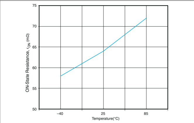
Figure 7-2. r_{ON} vs Temperature ( V_{IN} = 3.3 V)
