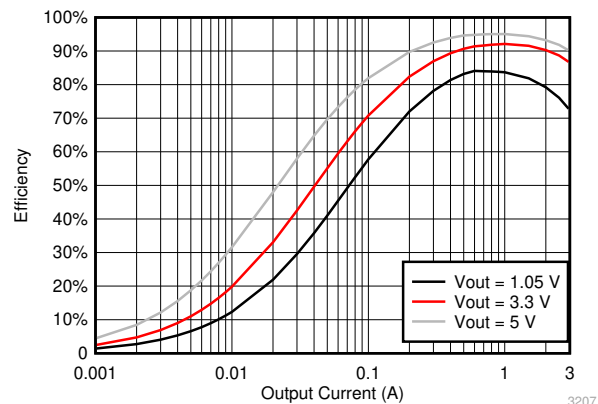
TPS563207 Efficiency
