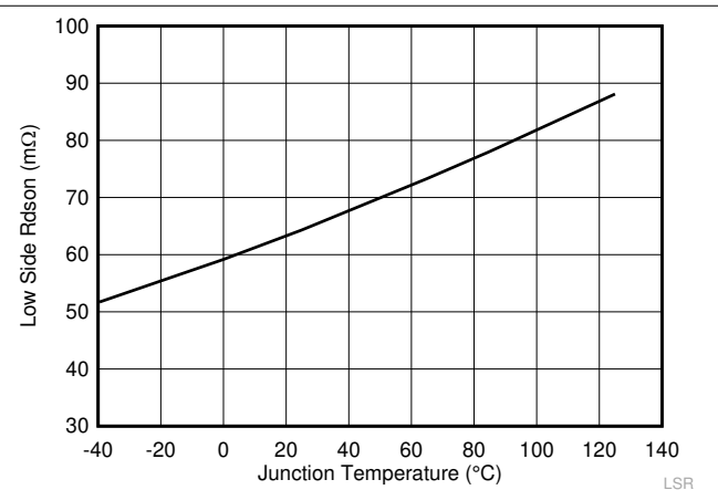
Figure 7-6. Low-Side R_{ds-On} vs Junction Temperature
