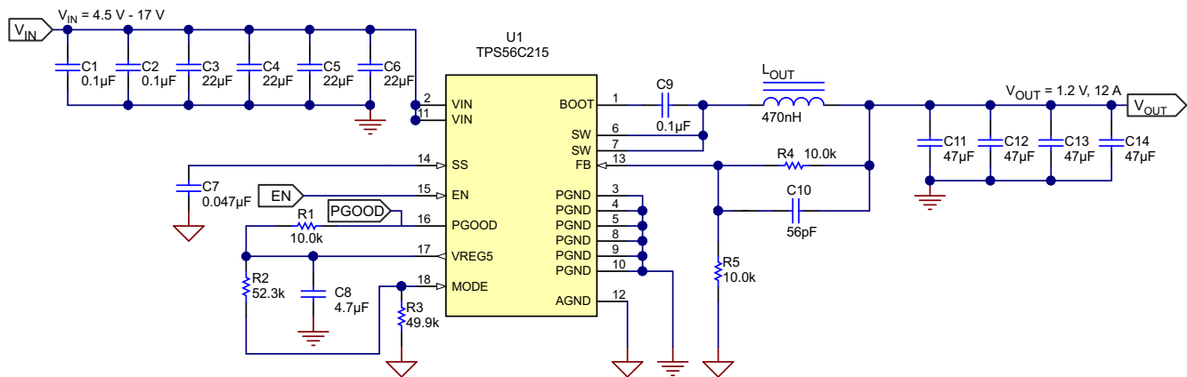
Figure 7-1. Application Schematic
