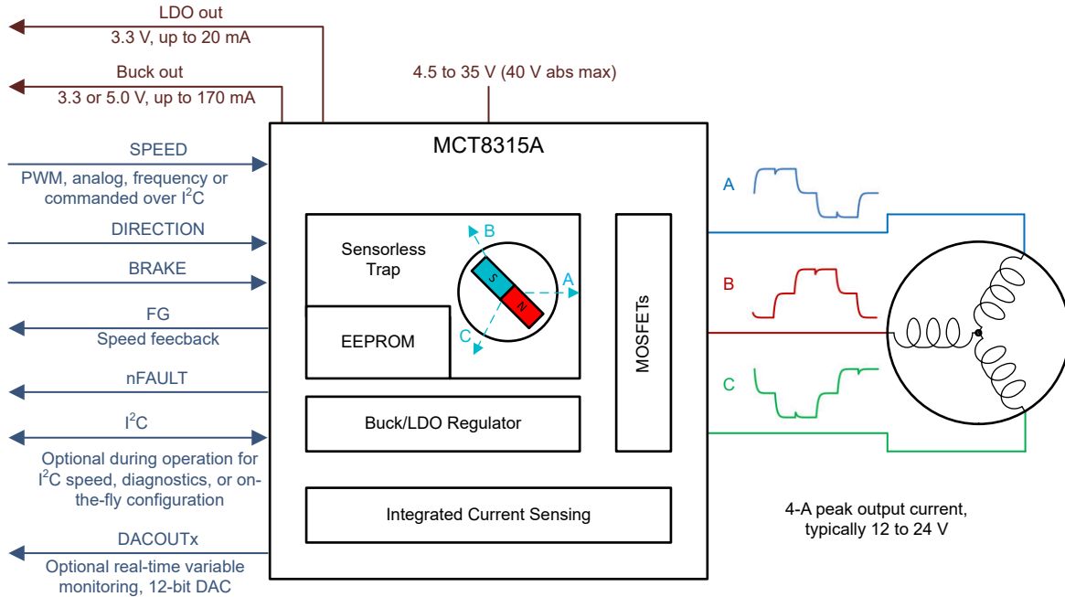
Figure 2-1. Simplified Schematic of MCT8315A
