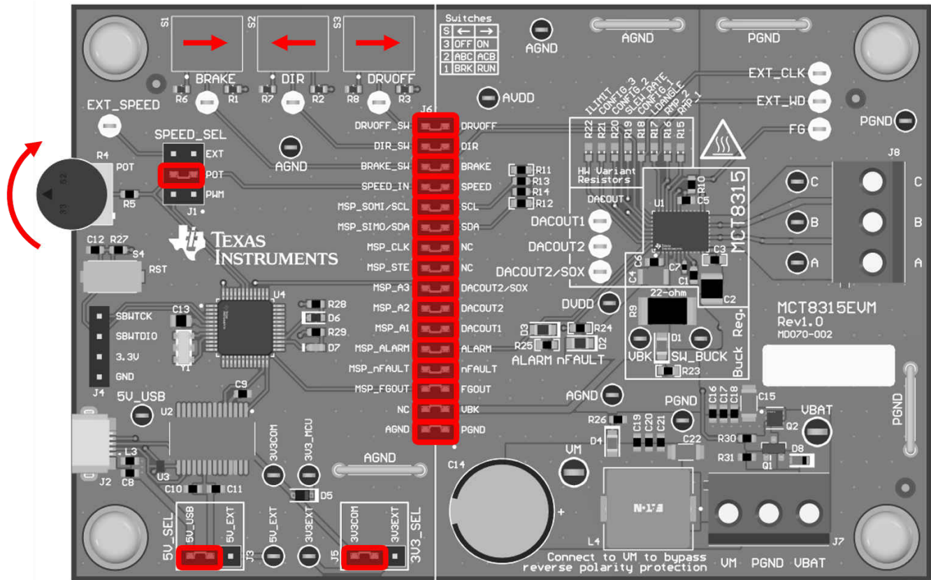
Figure 2-2. MCT8315EVM Jumper Configuration
