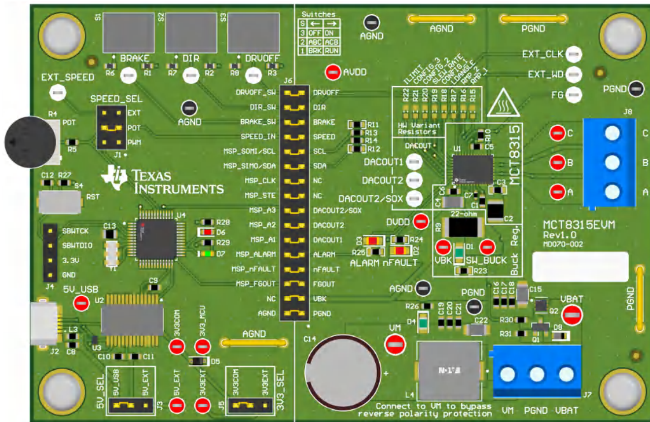
Figure 2-3. MCT8315EVM External Configuration
