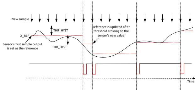
Figure 4. TMAG3001 Wake on Change with Magnetic Axes Measurements
