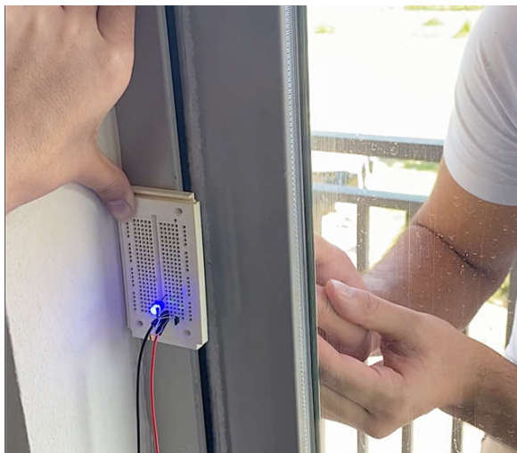
Figure 2. Tamper Test Setup
