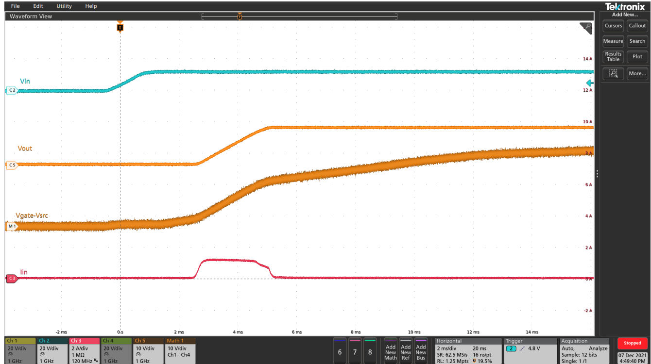
Figure 5-3. Startup with 220- \mu F Cout
