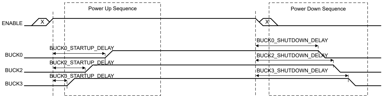
Figure 2-1. Generic Startup and Shutdown Sequences of the Regulators
