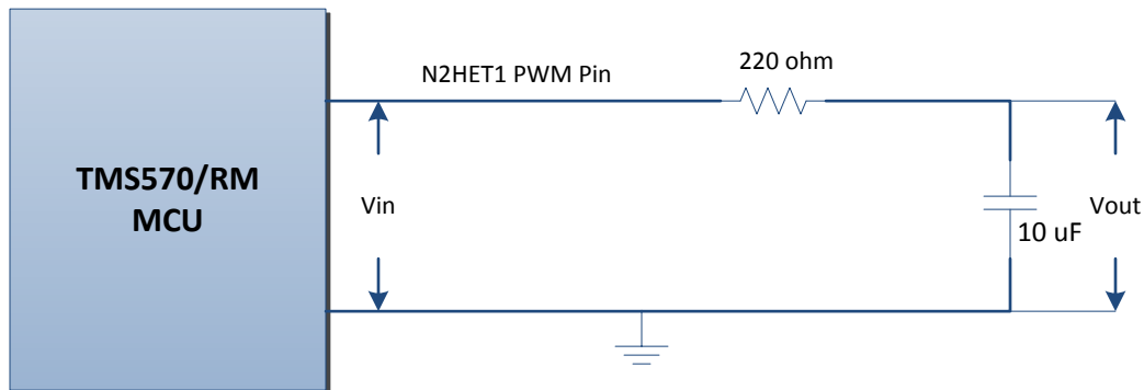
Figure 4. Low-Pass Filter
