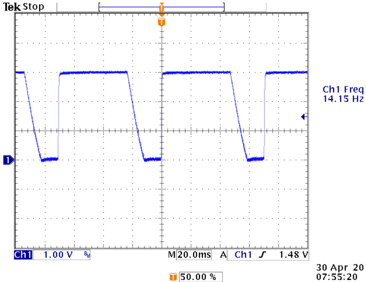
Figure 12. A Right Trapezoid
