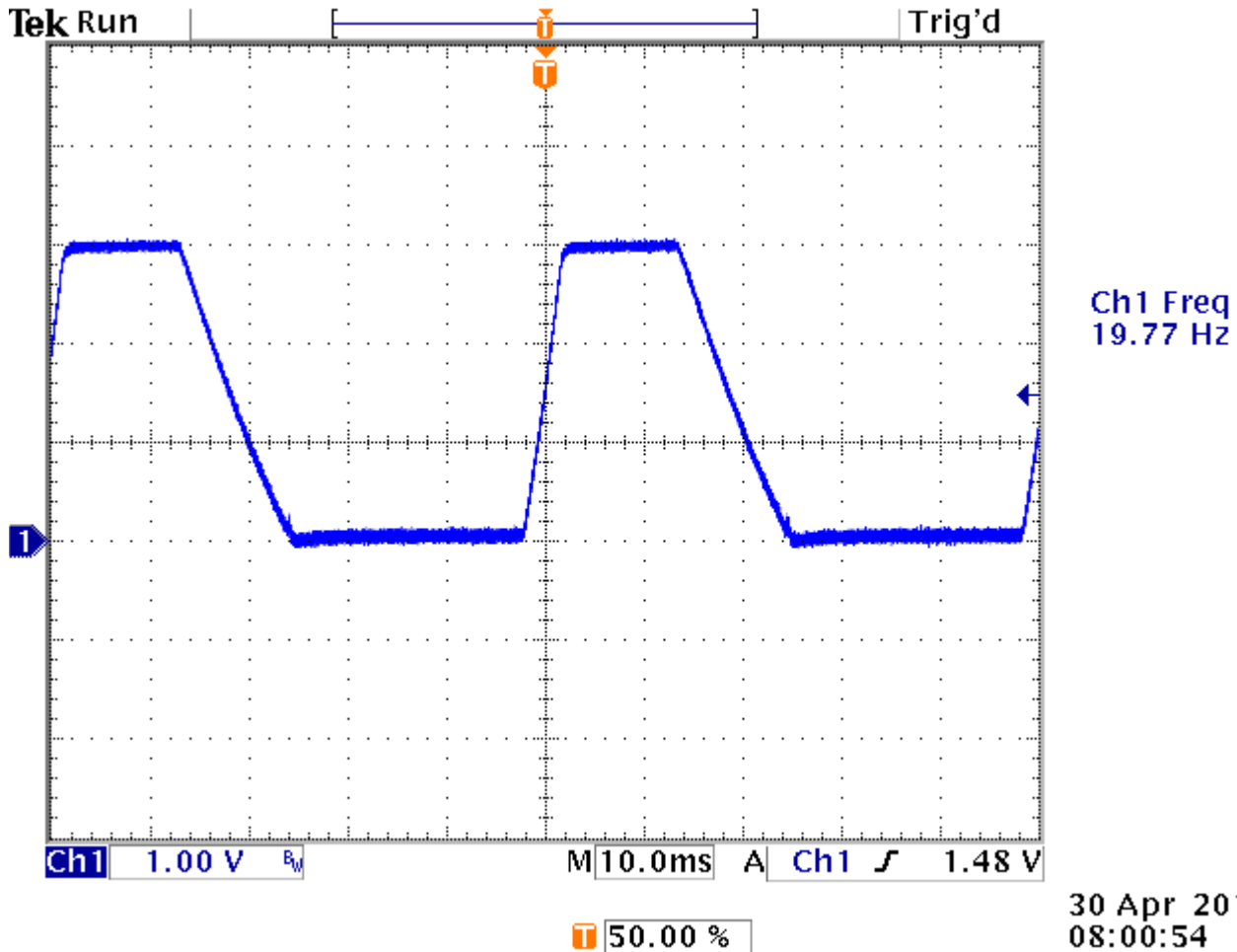
Figure 13. A Scalene Trapezoid
