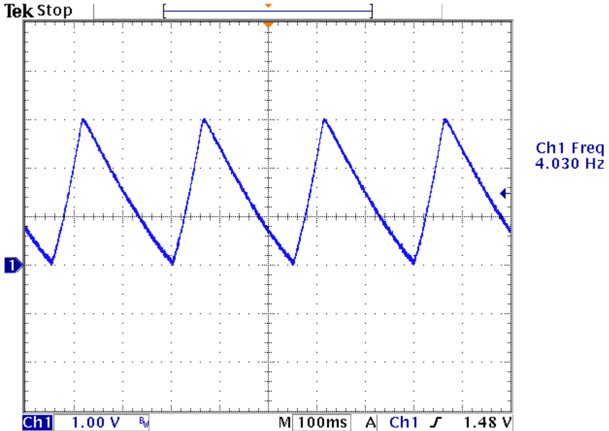
Figure 9. A Scalene Triangle
