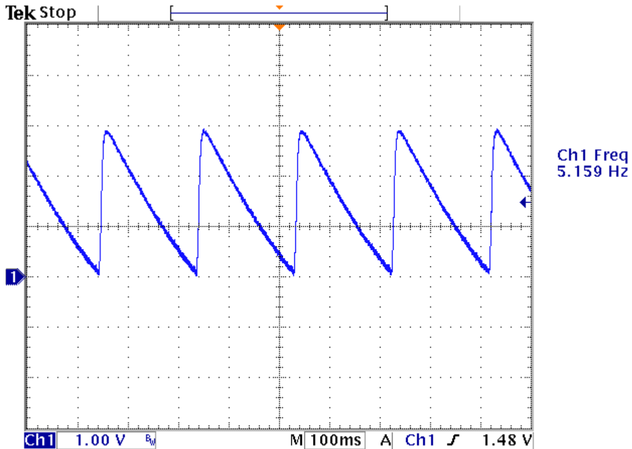
Figure 10. A Sawtooth Triangle
