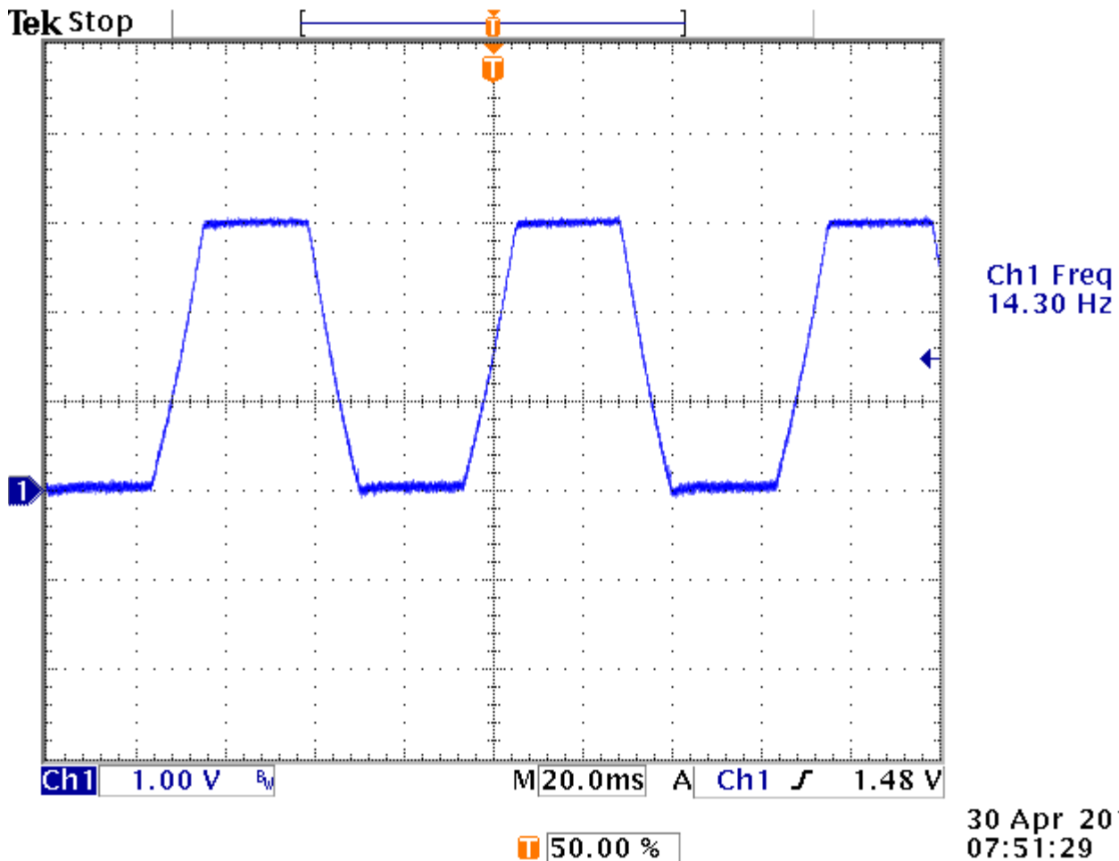
Figure 11. An Isosceles Trapezoid
