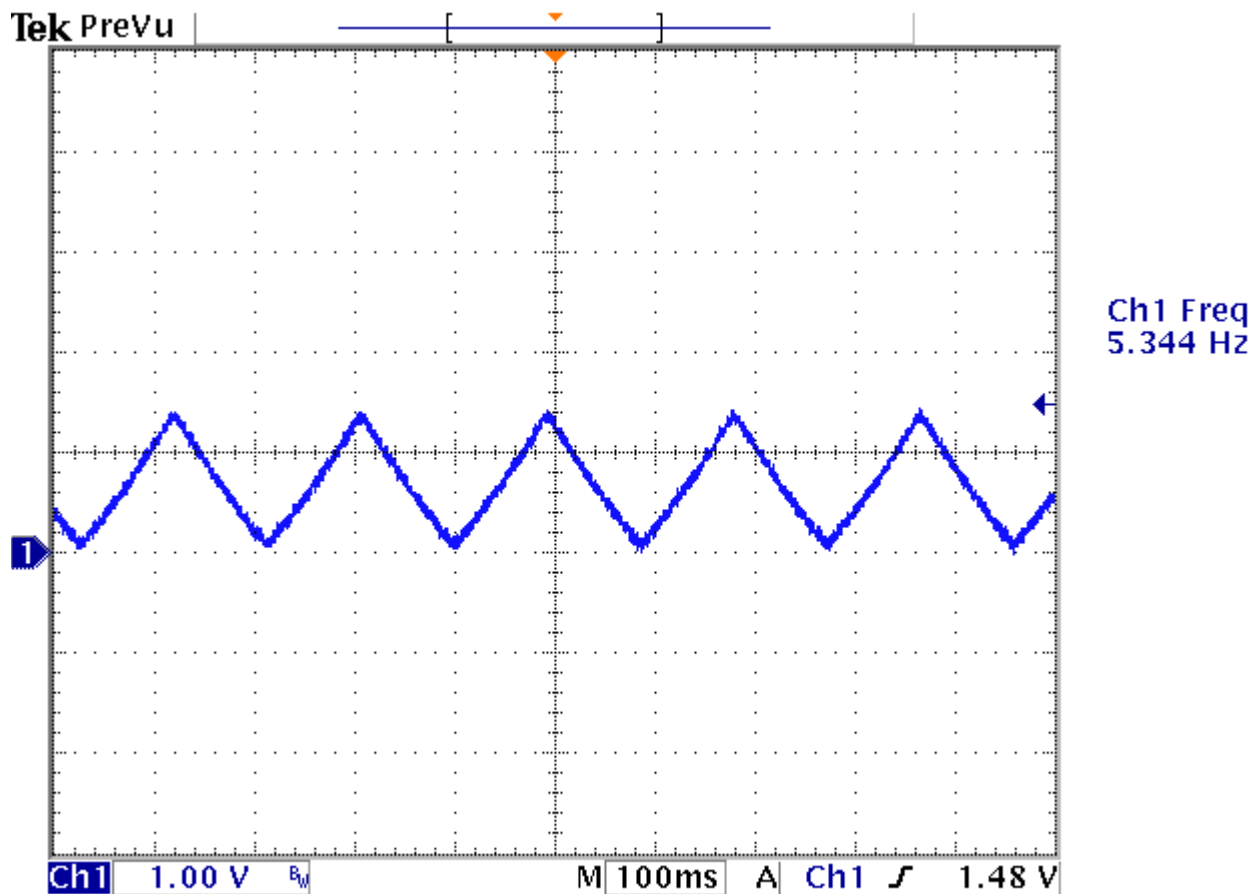
Figure 8. An Isosceles Triangle 2
