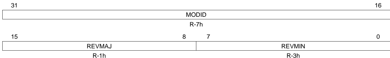
Figure 14. MDIO Version Register (VERSION)
