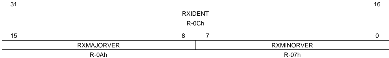
Figure 31. Receive Identification and Version Register (RXIDVER)
