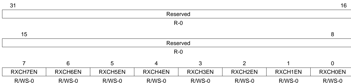
Figure 48. Receive Unicast Enable Set Register (RXUNICASTSET)
