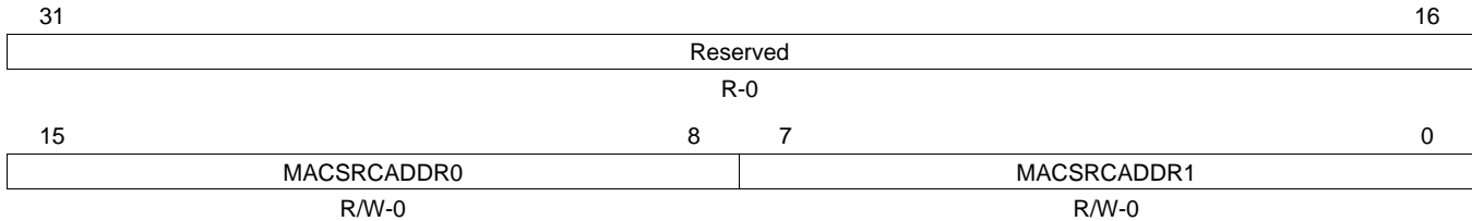
Figure 61. MAC Source Address Low Bytes Register (MACSRCADDRLO)
