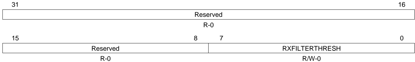
Figure 52. Receive Filter Low Priority Frame Threshold Register (RXFILTERLOWTHRESH)
