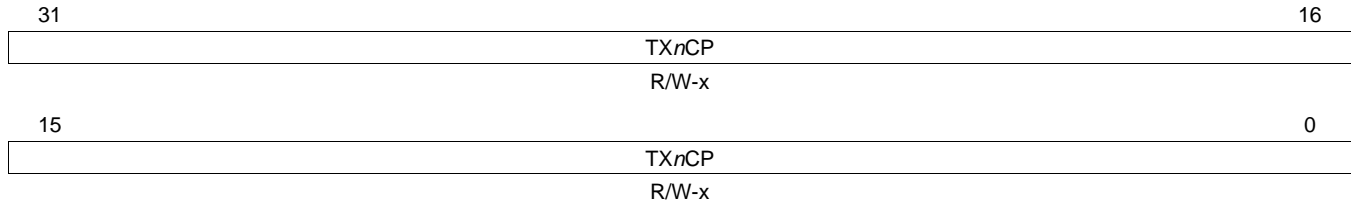
Figure 74. Transmit Channel n Completion Pointer Register (TX n CP)
