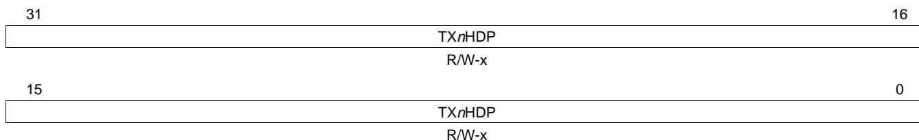
Figure 72. Transmit Channel n DMA Head Descriptor Pointer Register (TXnHDP)
