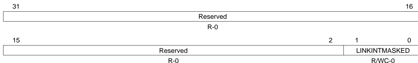
Figure 19. MDIO Link Status Change Interrupt (Masked) Register (LINKINTMASKED)
