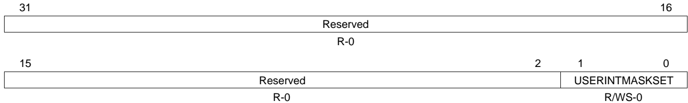
Figure 22. MDIO User Command Complete Interrupt Mask Set Register (USERINTMASKSET)
