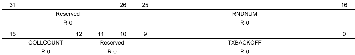
Figure 65. Back Off Random Number Generator Test Register (BOFFTEST)
