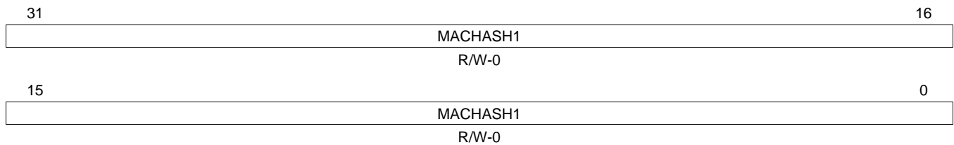
Figure 63. MAC Hash Address Register 1 (MACHASH1)
