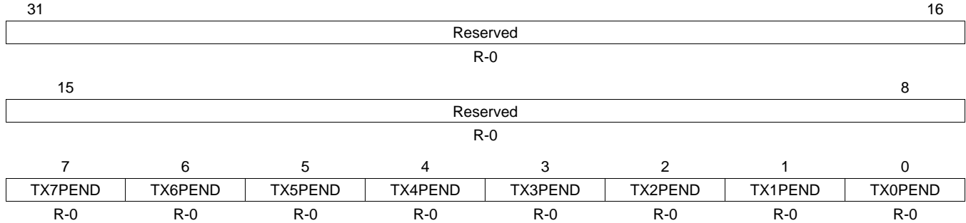
Figure 35. Transmit Interrupt Status (Masked) Register (TXINTSTATMASKED)
