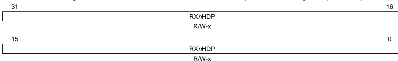
Figure 73. Receive Channel n DMA Head Descriptor Pointer Register (RXnHDP)
