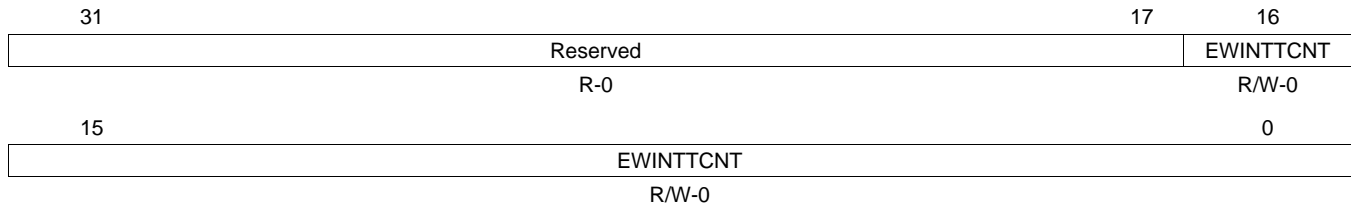
Figure 13. EMAC Control Module Interrupt Timer Count Register (EWINTTCNT)
