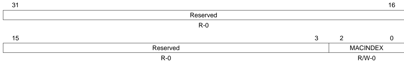
Figure 71. MAC Index Register (MACINDEX)
