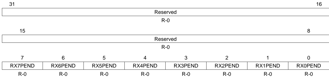
Figure 40. Receive Interrupt Status (Masked) Register (RXINTSTATMASKED)
