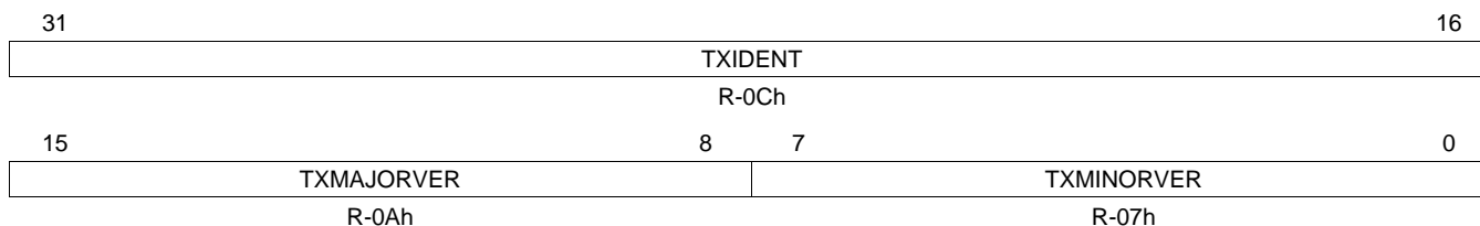
Figure 28. Transmit Identification and Version Register (TXIDVER)
