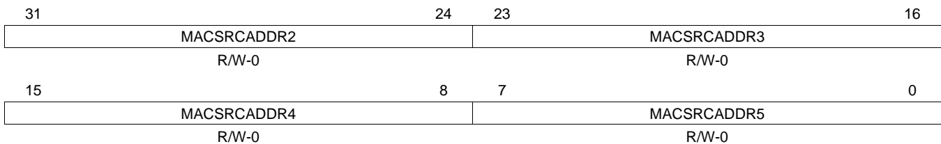
Figure 62. MAC Source Address High Bytes Register (MACSRCADDRHI)
