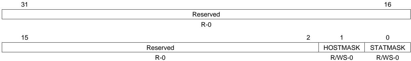
Figure 45. MAC Interrupt Mask Set Register (MACINTMASKSET)
