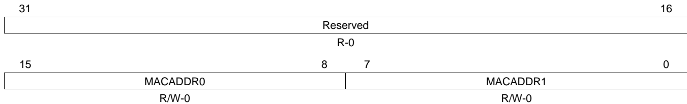
Figure 69. MAC Address Low Bytes Register (MACADDRLO)
