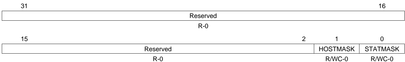
Figure 46. MAC Interrupt Mask Clear Register (MACINTMASKCLEAR)
