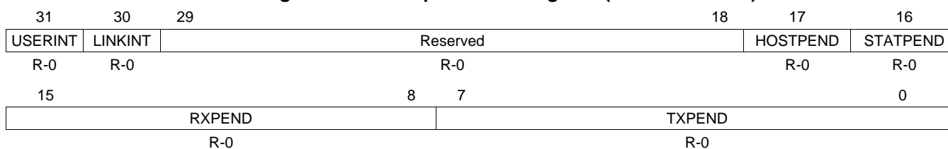
Figure 38. MAC Input Vector Register (MACINVECTOR)
