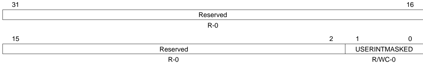
Figure 21. MDIO User Command Complete Interrupt (Masked) Register (USERINTMASKED)
