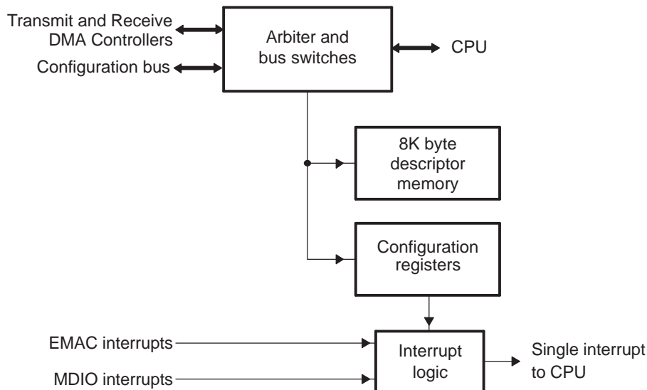
Figure 9. EMAC Control Module Block Diagram
