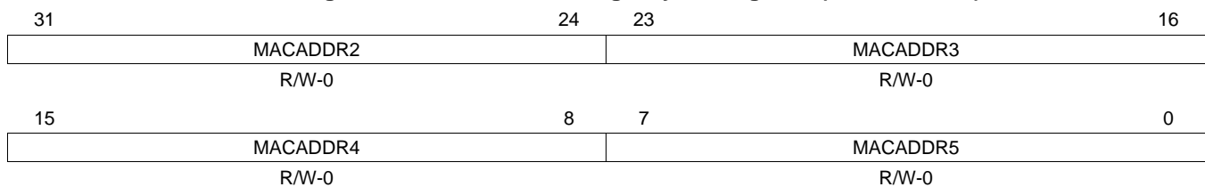
Figure 70. MAC Address High Bytes Register (MACADDRHI)
