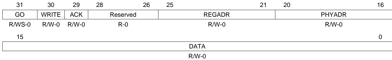
Figure 24. MDIO User Access Register 0 (USERACCESS0)
