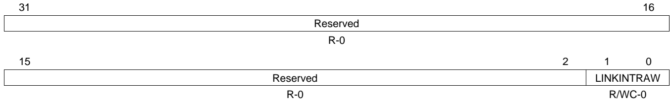
Figure 18. MDIO Link Status Change Interrupt (Unmasked) Register (LINKINTRAW)
