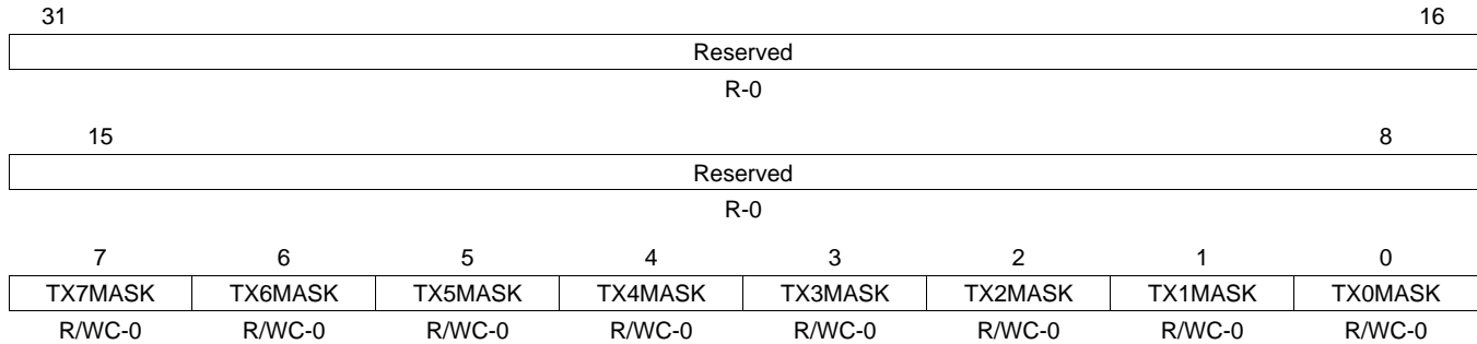
Figure 37. Transmit Interrupt Mask Clear Register (TXINTMASKCLEAR)
