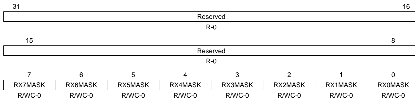
Figure 42. Receive Interrupt Mask Clear Register (RXINTMASKCLEAR)
