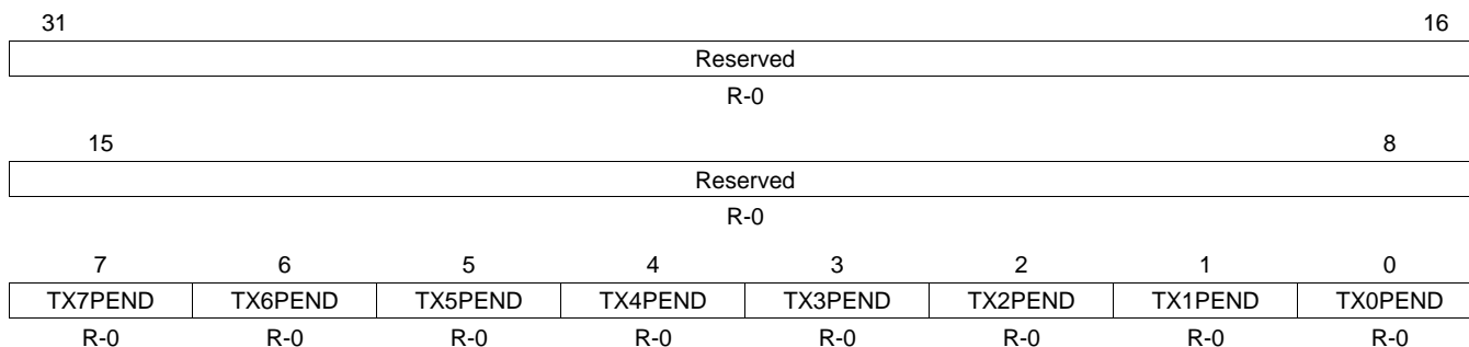
Figure 34. Transmit Interrupt Status (Unmasked) Register (TXINTSTATRAW)
