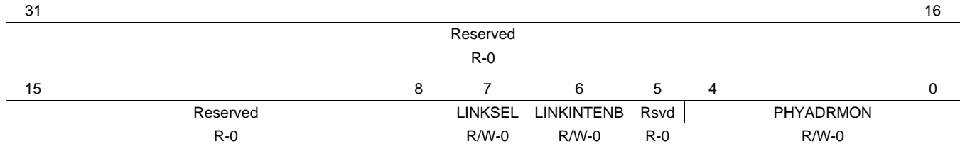
Figure 25. MDIO User PHY Select Register 0 (USERPHYSEL0)
