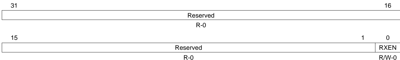
Figure 32. Receive Control Register (RXCONTROL)
