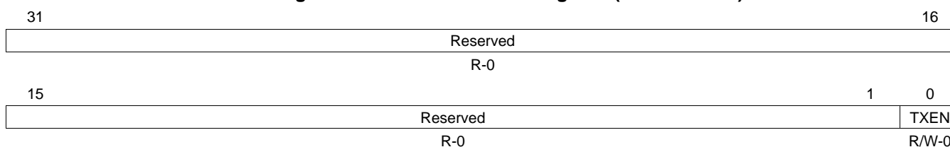
Figure 29. Transmit Control Register (TXCONTROL)
