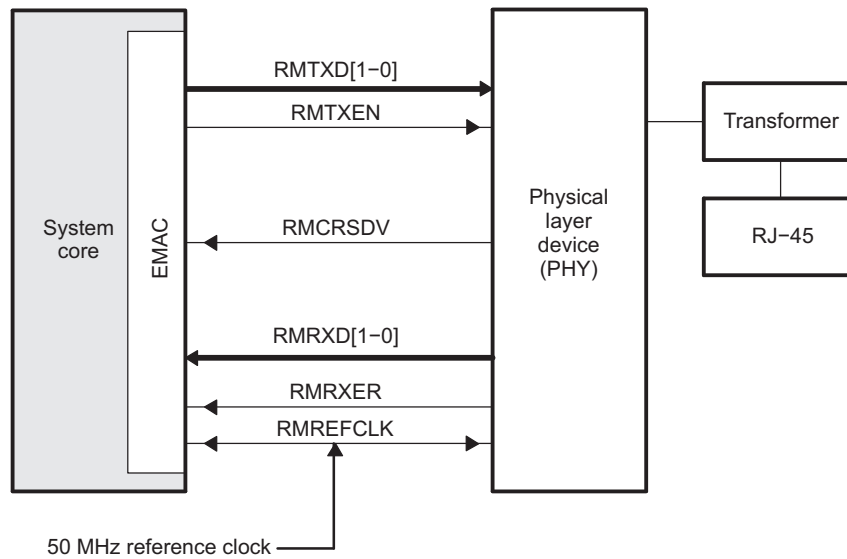
Figure 3. Ethernet Configuration with RMI Interface
