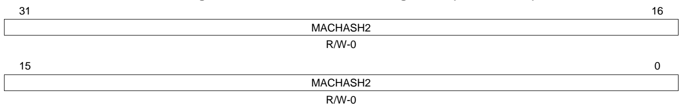
Figure 64. MAC Hash Address Register 2 (MACHASH2)
