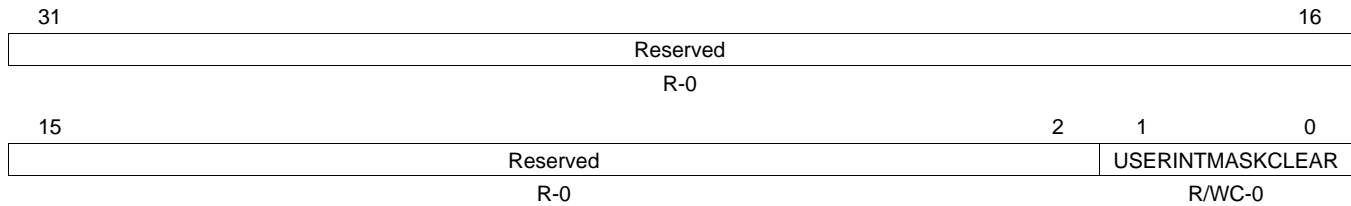
Figure 23. MDIO User Command Complete Interrupt Mask Clear Register (USERINTMASKCLEAR)
