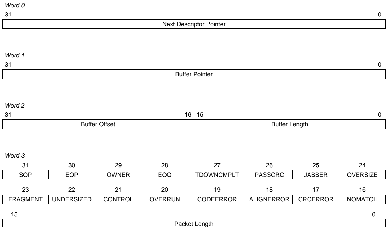
Figure 8. Receive Buffer Descriptor Format
