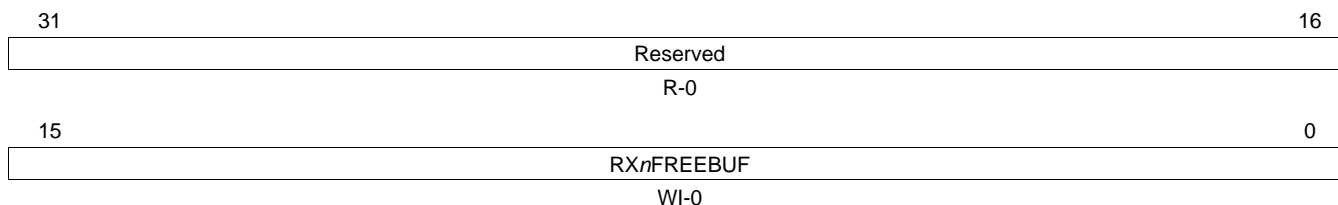
Figure 54. Receive Channel n Free Buffer Count Register (RX n FREEBUFFER)
