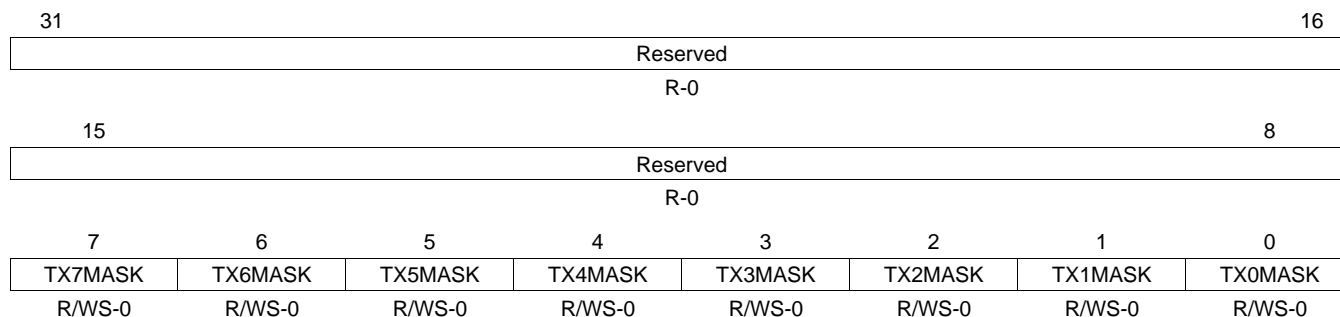
Figure 36. Transmit Interrupt Mask Set Register (TXINTMASKSET)
