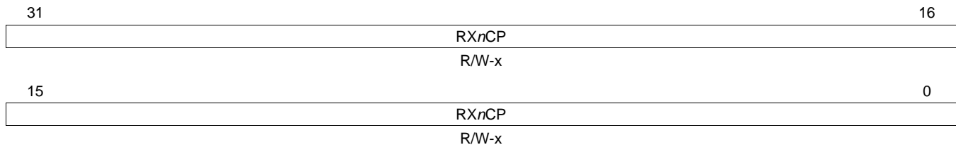
Figure 75. Receive Channel n Completion Pointer Register (RX n CP)
