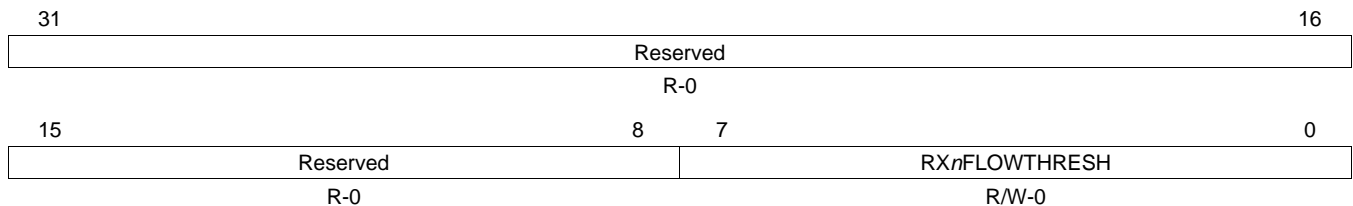
Figure 53. Receive Channel n Flow Control Threshold Register (RX n FLOWTHRESH)
