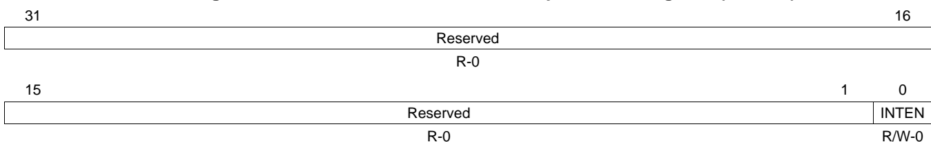
Figure 12. EMAC Control Module Interrupt Control Register (EWCTL)
