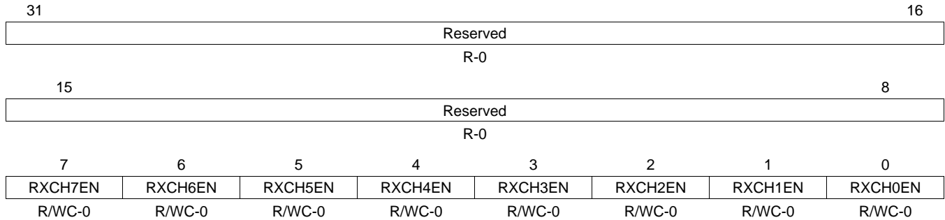
Figure 49. Receive Unicast Clear Register (RXUNICASTCLEAR)
