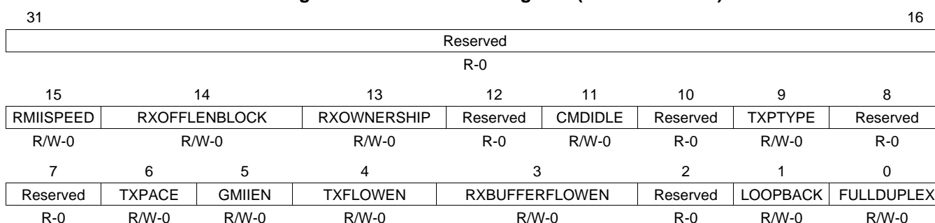
Figure 55. MAC Control Register (MACCONTROL)
