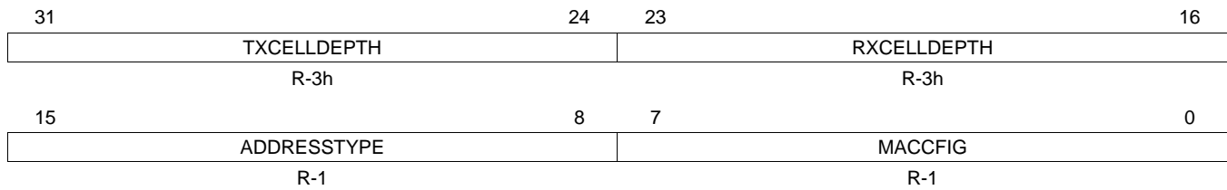
Figure 59. MAC Configuration Register (MACCONFIG)
