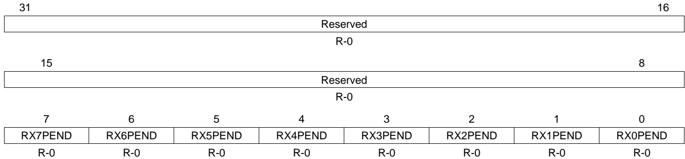
Figure 39. Receive Interrupt Status (Unmasked) Register (RXINTSTATRAW)
