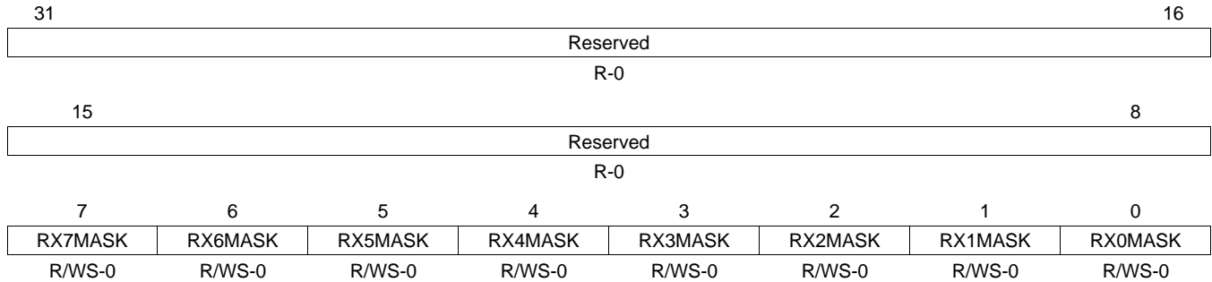
Figure 41. Receive Interrupt Mask Set Register (RXINTMASKSET)
