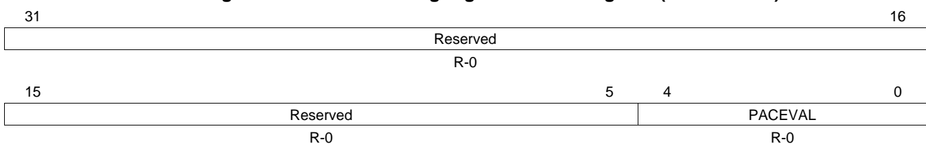
Figure 66. Transmit Pacing Algorithm Test Register (TPACETEST)
