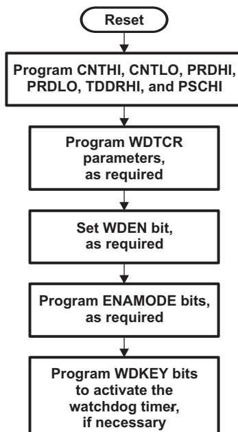
Figure 10. Timer Initialization
