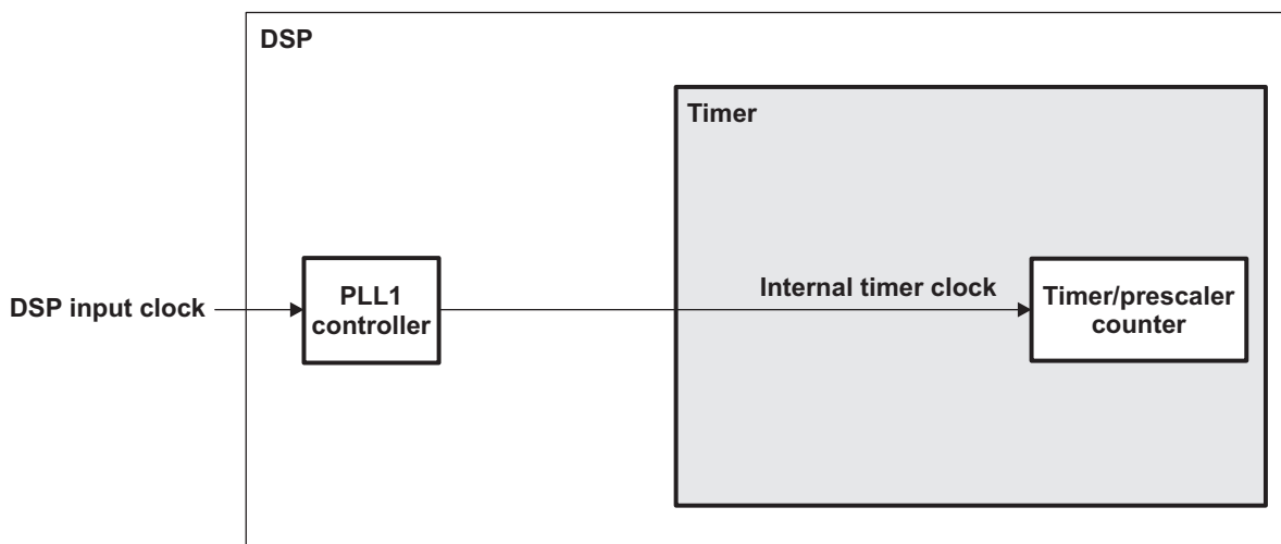
Figure 2. Generation of the Internal Timer Clock
