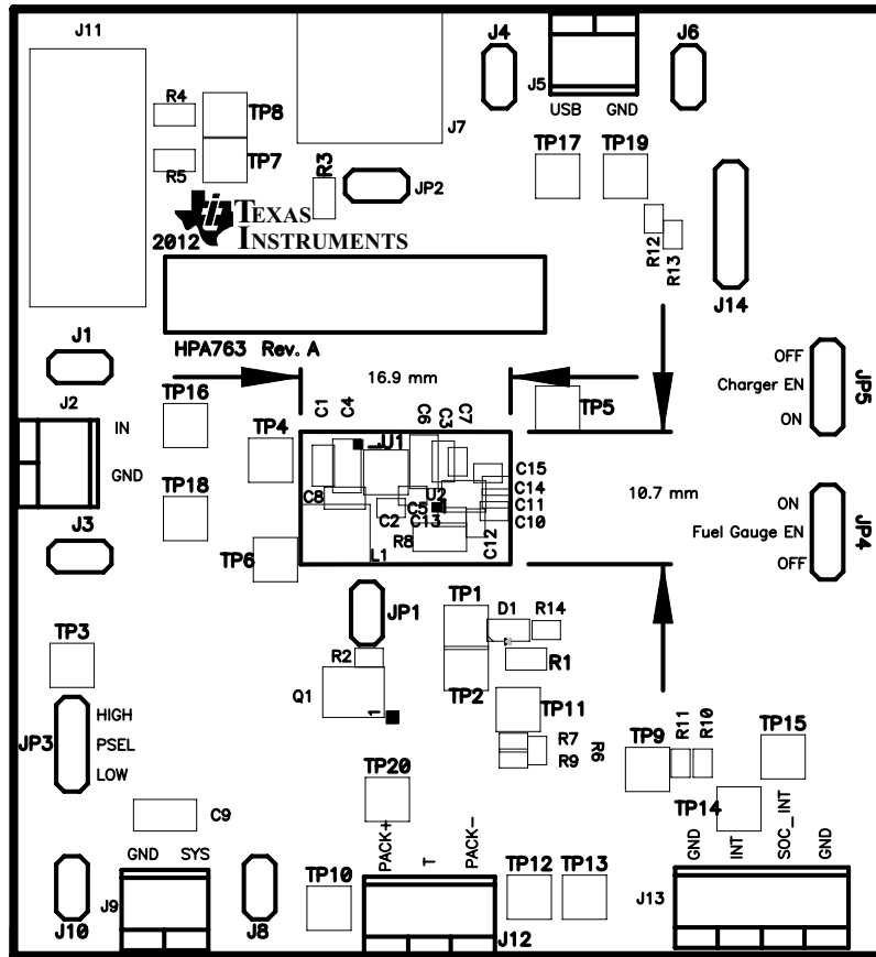
Figure 2. bq27530EVM-001 Layout – Layer 1 Silk Screen
