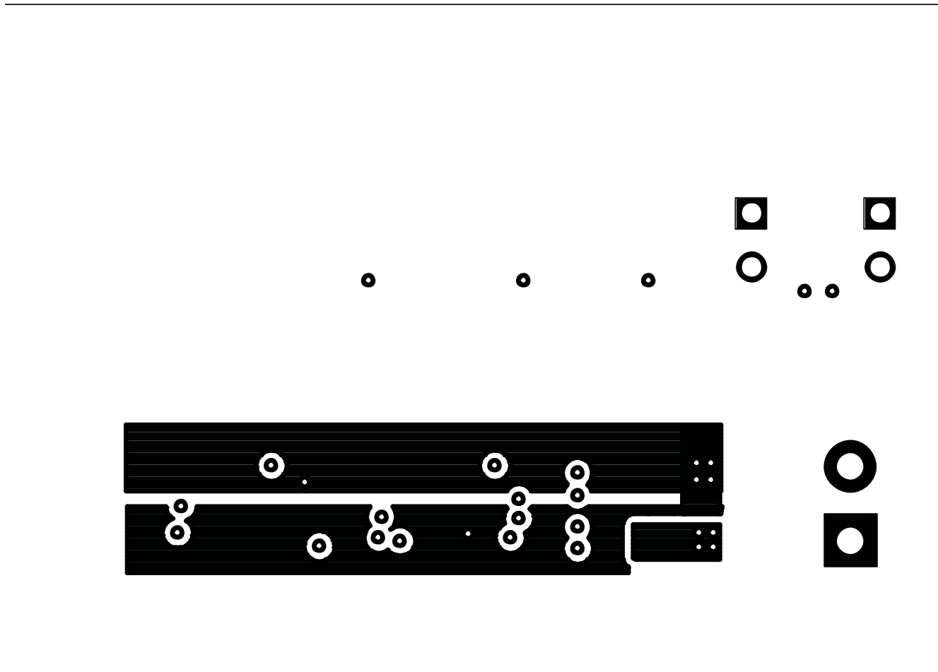
Figure 5. bq27x10EVM Layer 2 Layout
